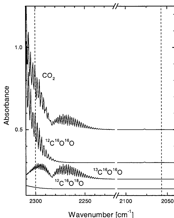
Figure 2. Optimal spectral window (bounded by dashed lines) for ^{12}\text{CO}_2 , ^{13}\text{CO}_2 , and hence \delta^{13}\text{CO}_2 analysis, 2300\text{--}2060 \text{ cm}^{-1} .
