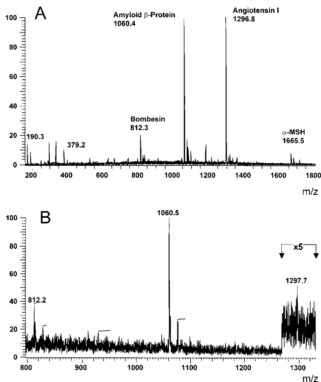
Figure 2. AP MALDI spectrum of the four-peptide mixture, obtained by deposition of 0.75 \mu\text{L} of analyte solution and 0.75 \mu\text{L} of matrix ( \alpha -cyano-4-hydroxycinnamic acid, HP matrix solution): (A) 50 and (B) 5 \text{pg}/\mu\text{L} of each peptide.
