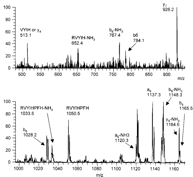
Figure 4. \text{MS}^3 spectrum of four peptide mixture (0.5 \text{ng}/\mu\text{L} of each peptide) at m/z 1297.5 \rightarrow 1165.5 \rightarrow . The peak at m/z 1165.5 was collected within a range of \pm 1.5 Da. Thus, \text{MS}^3 was performed on both the b_9 and the y_9 - \text{NH}_3 ions.
