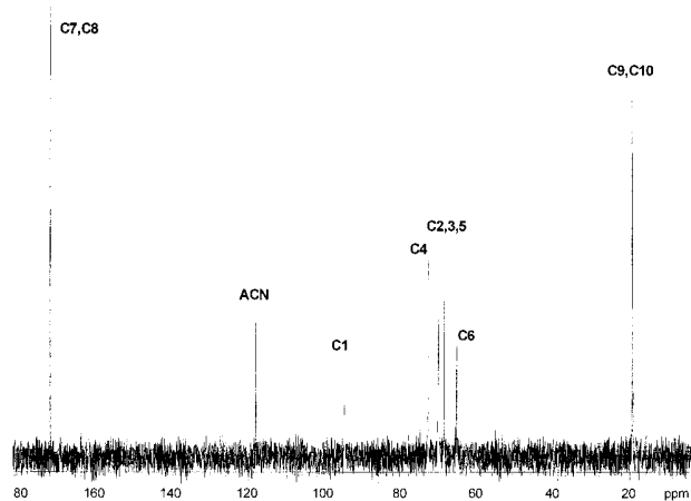
Figure 7. 300 MHz ^{13}\text{C} NMR spectrum of ODAS- \gamma CD. Solvent: \text{D}_2\text{O} . C1–C6: respective carbon atoms in the glucose moieties. C7,8: CO carbon atoms in the acetyl functional groups connected to the C2, C3 carbons of the glucose moieties. C9,10: \text{CH}_3 carbon atoms in the acetyl functional groups connected to the C2, C3 carbons of the glucose moieties.
