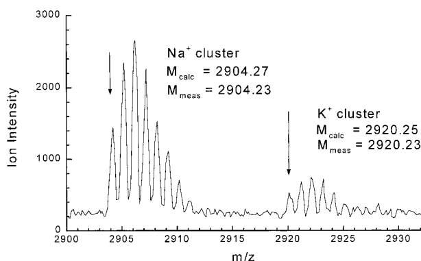
Figure 3. Partial mass spectrum of intermediate 3 obtained by MALDI-TOF-MS. For conditions see Experimental Section.
