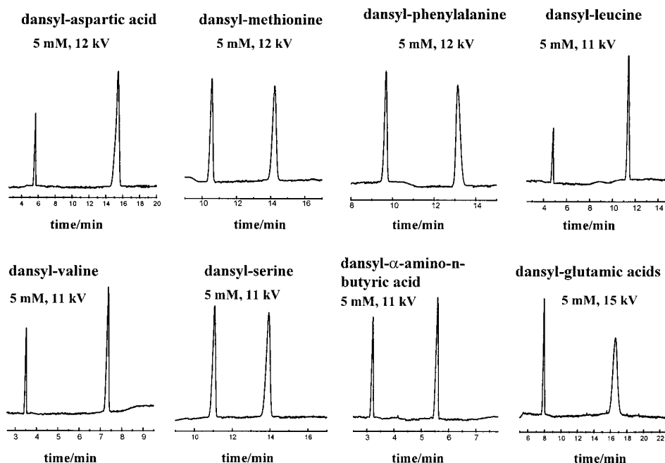
Figure 16. Typical electropherograms of chiral amphoteric analytes. The numbers next to the structures indicate the ODAS- \gamma CD concentrations (mM) and the applied effective potentials (kV). Capillary: 25 \mu m i.d. 19 cm/26 cm effective/total length, uncoated fused silica. Other conditions: see Experimental Section.
