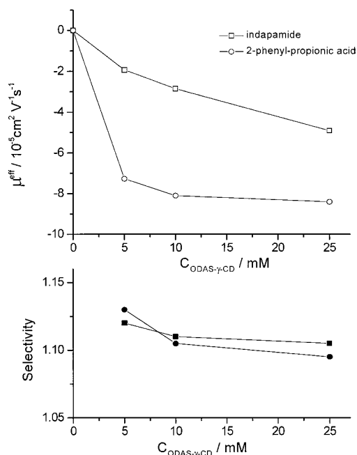
Figure 11. Effective mobilities (top panel, open symbols) and separation selectivities (bottom panel, filled symbols) for the weak-acid analytes as a function of the ODAS- \gamma -CD concentration. Symbols: square, indapamide; circle, 2-phenyl-propionic acid.
