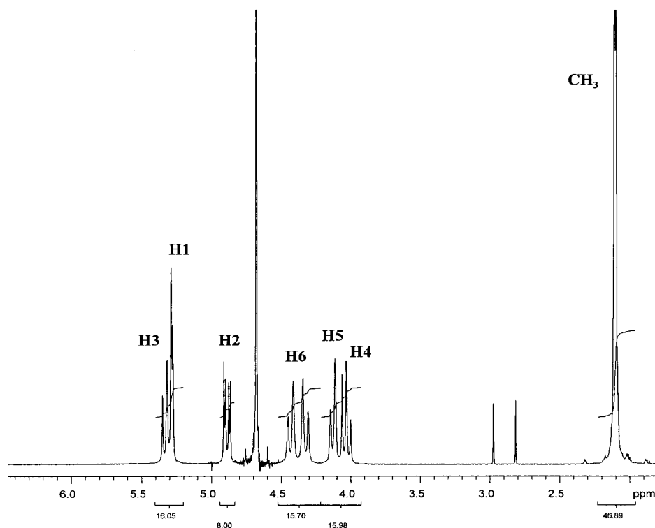
Figure 6. 300 MHz ^1\text{H} NMR spectrum of ODAS- \gamma -CD. Solvent: \text{D}_2\text{O} .
