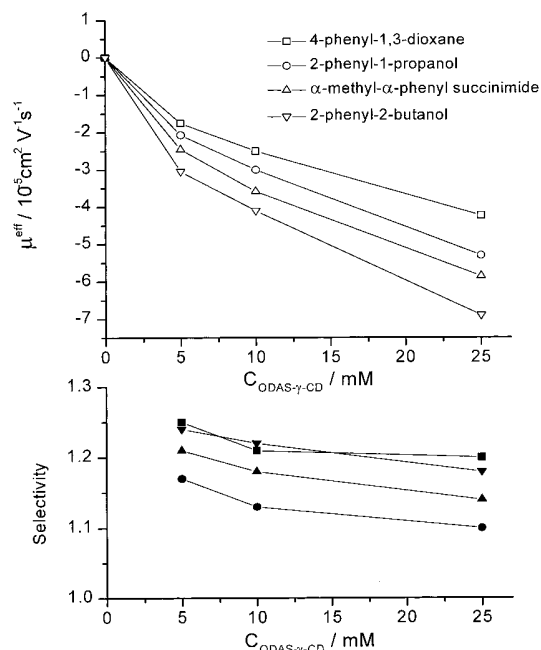
Figure 10. Effective mobilities (top panel, open symbols) and separation selectivities (bottom panel, filled symbols) for the non-charged analytes as a function of the ODAS- \gamma -CD concentration. Symbols: square, 4-phenyl-1,3-dioxane; circle, 2-phenyl-1-propanol; up-triangle, \alpha -methyl- \alpha -phenyl-succinimide; down-triangle, 2-phenyl-2-butanol.
