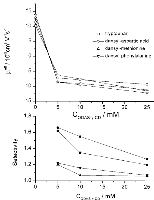
Figure 13. Effective mobilities (top panel, open symbols) and separation selectivities (bottom panel, filled symbols) for the amphoteric analytes as a function of the ODAS- \gamma -CD concentration. Symbols: square, tryptophan; circle, dansyl-aspartic acid; up-triangle, dansyl-methionine; down-triangle, dansyl-phenylalanine.
