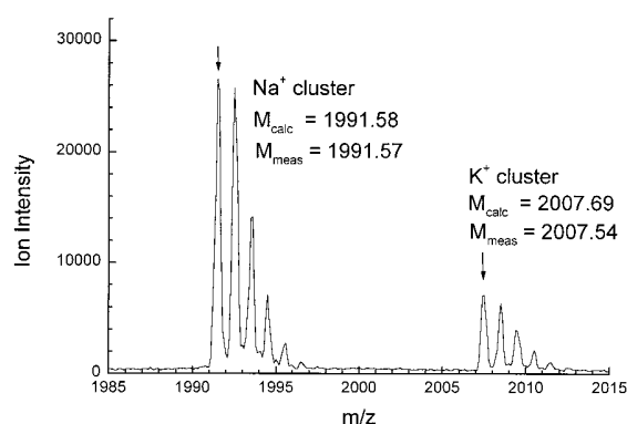
Figure 4. Partial mass spectrum of intermediate 4 obtained by MALDI-TOF-MS. For conditions see Experimental Section.
