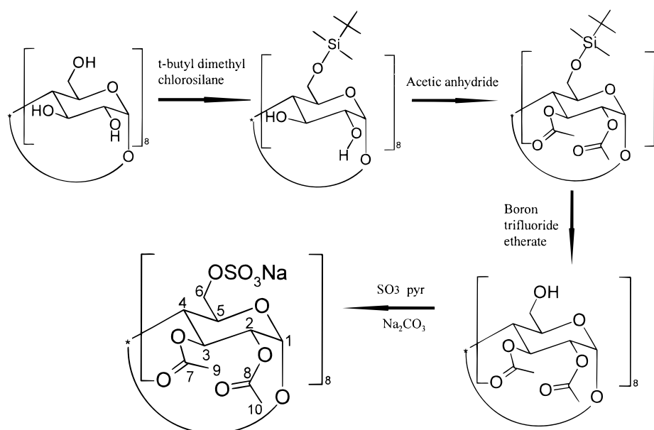
Figure 1. Synthesis scheme for octakis(2,3-diacetyl-6-sulfato)- \gamma -cyclodextrin.
