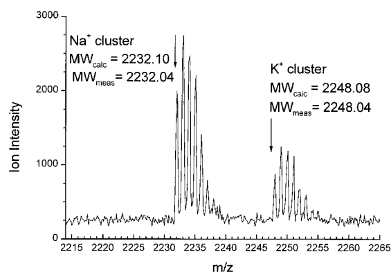
Figure 2. Partial mass spectrum of intermediate 2 obtained by MALDI-TOF-MS. For conditions see Experimental Section.
