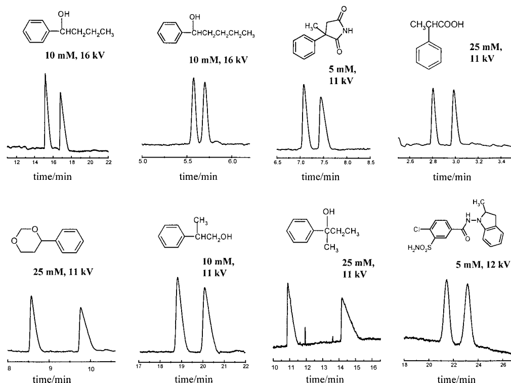
Figure 14. Typical electropherograms of chiral noncharged and weak-acid analytes. The numbers next to the structures indicate the ODAS- \gamma CD concentrations (mM) and the applied effective potentials (kV). Capillary: 25 \mu m i.d. 19 cm/26 cm effective/total length, uncoated fused silica. Other conditions: see Experimental Section.
