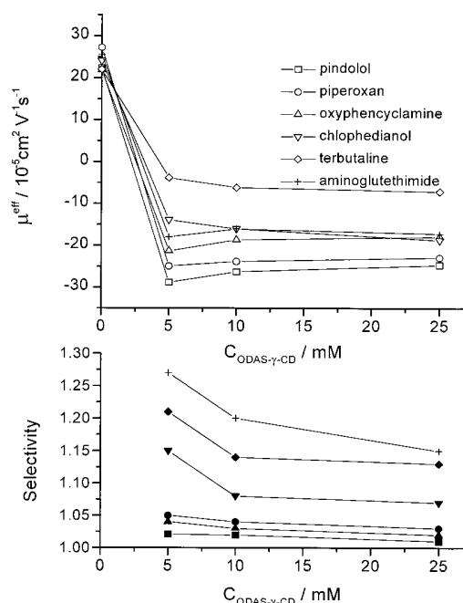
Figure 12. Effective mobilities (top panel, open symbols) and separation selectivities (bottom panel, filled symbols) for the weak-base analytes as a function of the ODAS- \gamma -CD concentration. Symbols: square, pindolol; circle, piperoxan; up-triangle, oxyphenyclamine; down-triangle, chlophedianol; cross, aminoglutethimide.
