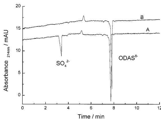
Figure 5. Indirect UV-detection electropherogram of ODAS- \gamma CD before (A) and after (B) removal of sodium sulfate. BE: 20 mM p -toluenesulfonic acid, pH 4.1 adjusted with \epsilon -aminocaproic acid. Wavelength: 214 nm. Applied potential: 10 kV. Thermostat temperature: 20 C. Capillary: 25- \mu\text{m} i.d. 39 cm/46 cm effective/total length, uncoated fused silica.
