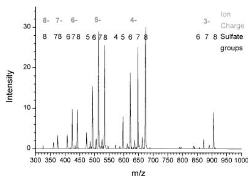
Figure 8. Mass spectrum of ODAS- \gamma CD obtained by ESI-MS. For conditions see Experimental Section.
