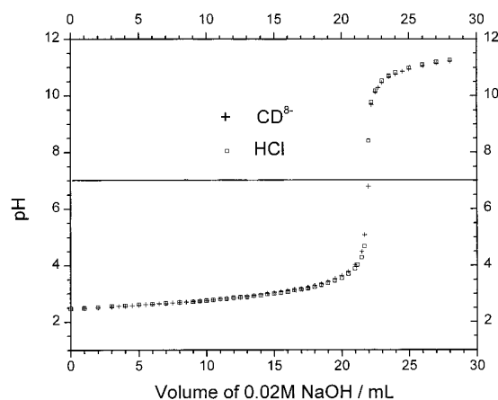
Figure 9. Potentiometric titration curves for 0.058 mmol ODAS- \gamma CD and 0.46 mmol HCl.
