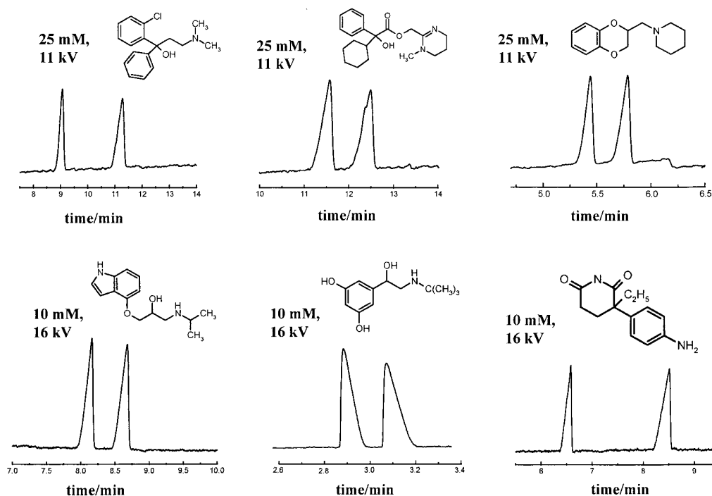
Figure 15. Typical electropherograms of chiral weak base analytes. The numbers next to the structures indicate the ODAS- \gamma CD concentrations (mM) and the applied effective potentials (kV). Capillary: 25 \mu m i.d. 19 cm/26 cm effective/total length, uncoated fused silica. Other conditions: see Experimental Section.
