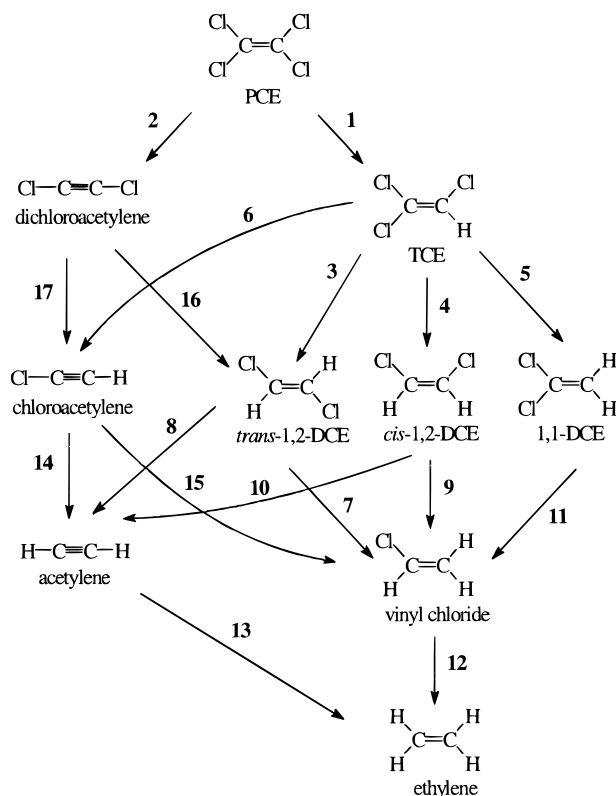
FIGURE 1. Hypothesized reaction sequence (1, 15) for reduction of chlorinated ethylenes and related compounds. Reaction numbers correspond to rate constants given in Table 1.
