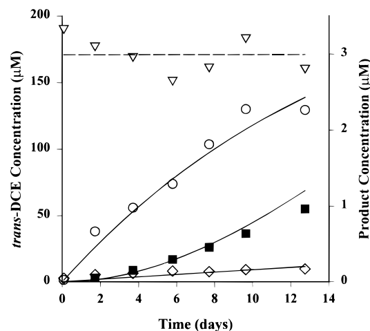
FIGURE 2. Reduction of trans -DCE ( \nabla ) by 25 g of Zn(0) in 160 mL of 0.1 M NaCl/0.05 M Tris buffer (pH 7.2). Solid lines are model fits to reaction products acetylene ( \circ ), ethylene ( \blacksquare ), and vinyl chloride ( \diamond ). The dashed line represents the mean concentration of trans -DCE determined by averaging the data points shown.
