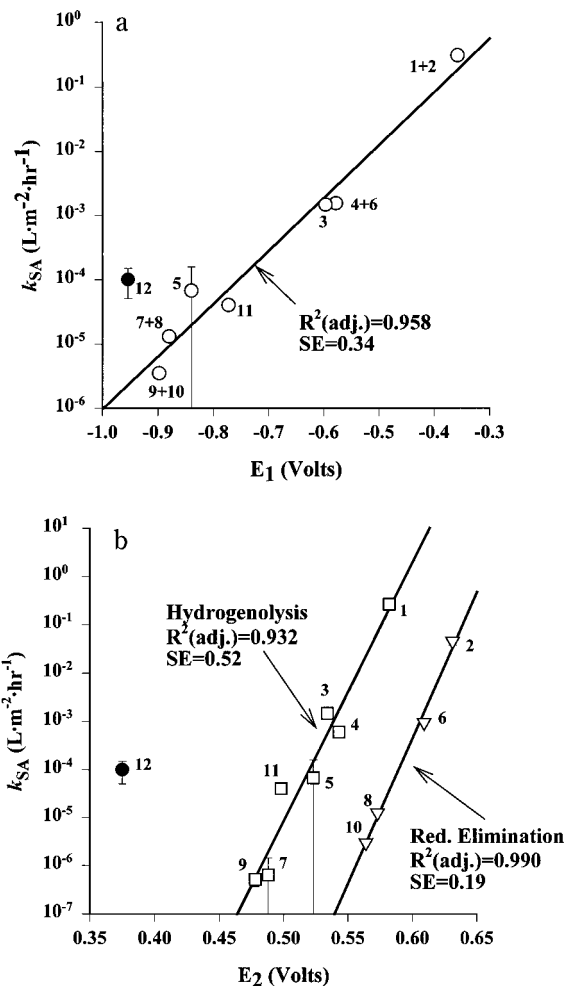
FIGURE 7. Correlation of surface area-normalized rate constants ( k_{SA} , Table 1) (a) with one-electron reduction potentials and (b) with two-electron reduction potentials. Numbering corresponds to the reactions indicated in Table 1. Regression lines exclude the data point for vinyl chloride (filled circle, reaction 12). If no error bar is shown, it is smaller than the symbol.
