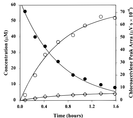
FIGURE 5. Reduction of chloroacetylene in 0.1 M NaCl/0.05 M Tris buffer (pH 7.2) by 1 g of Zn(0). Solid symbols ( \bullet ) represent chloroacetylene peak areas, while open symbols for acetylene ( \circ ) and vinyl chloride ( \diamond ) reflect measured concentrations. The model fit for the chloroacetylene data represents model-calculated concentrations.
