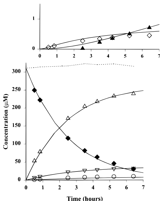
FIGURE 4. Reduction of PCE ( \blacklozenge ) in 150 mL of 0.1 M NaCl/0.05 M Tris buffer (pH 7.2) by 5 g of Zn(0). Major products are TCE ( \Delta ), trans -DCE ( \nabla ), and acetylene ( \circ ). Inset shows trace products cis -DCE ( \blacktriangle ) and vinyl chloride ( \diamond ). The dotted line represents the observed C_2 mass balance, while solid lines are model fits.
