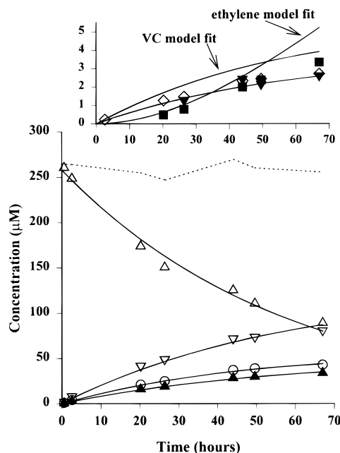
FIGURE 3. Reduction of TCE ( \Delta ) in 160 mL of 0.1 M NaCl/0.05 M Tris buffer (pH 7.2) by 25 g of Zn(0). Major products are trans -DCE ( \nabla ), acetylene ( \circ ), and cis -DCE ( \blacktriangle ). Inset shows trace products 1,1-DCE ( \blacktriangledown ), ethylene ( \blacksquare ), and vinyl chloride ( \diamond ). The dotted line represents the observed C_2 mass balance, while solid lines are model fits.
