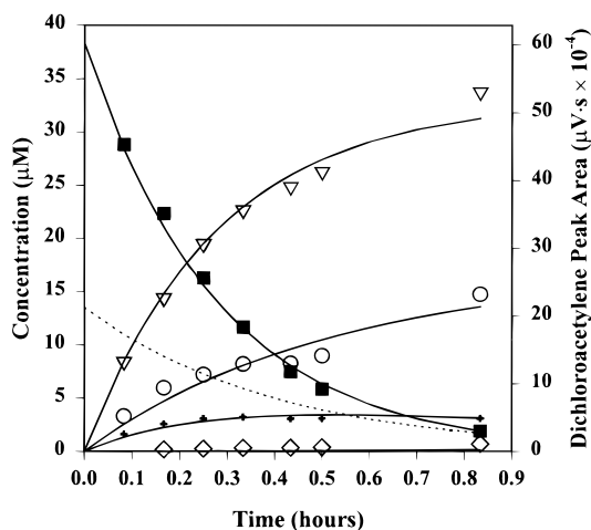
FIGURE 6. Reduction of dichloroacetylene in 0.1 M NaCl/0.05 M Tris buffer (pH 7.2) by 0.5 g of Zn(0). Solid symbols (■) represent dichloroacetylene peak areas. The model fit for the dichloroacetylene data represents model-calculated concentrations. Open symbols for trans -DCE (▽), acetylene (○), and vinyl chloride (◇) are measured concentrations. The chloroacetylene concentration (+) was calculated using the relationship between peak area and aqueous concentration developed in Figure 5. The dashed line represents the calculated concentration of a hypothesized contaminant assumed to react to form acetylene.
