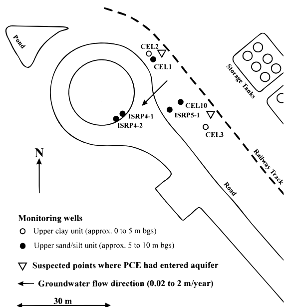
FIGURE 1. Plan of the field site at Toronto, Ontario, Canada.
