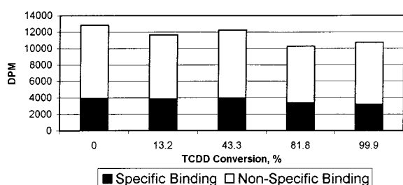
FIGURE 5. Specific and nonspecific binding of [ 3 H]estradiol for the estrogen receptor when competed against photolysis products 2,3,7,8-TCDD.
