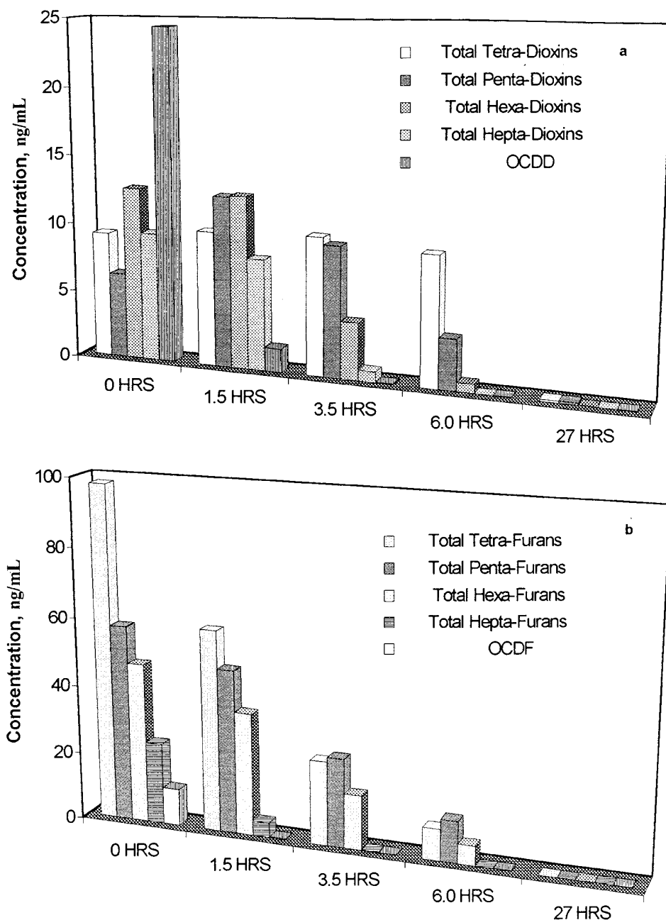
FIGURE 2. Change in concentrations (congener totals) of PCDD (a) and PCDF (b) during photolysis of the low-strength waste at 254 nm.
