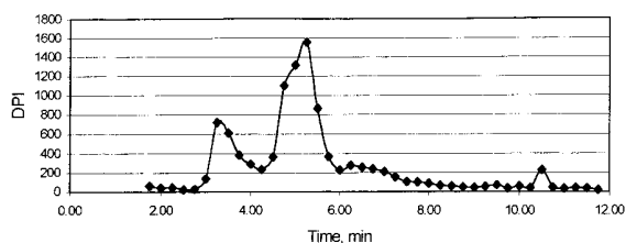
FIGURE 3. HPLC radiochromatogram from photolysis of 1,6-[ 3 H]-2,3,7,8-TCDD in hexane at 300 nm: mobile phase, 100% MeOH flow rate, 1 mL/min.
