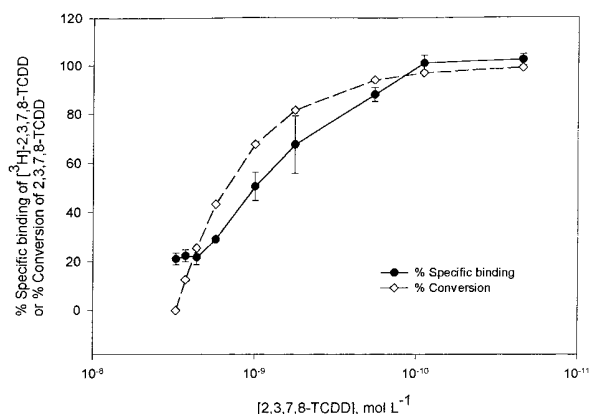
FIGURE 4. Relationship between percent specific binding of 1,6- 3 H-2,3,7,8-TCDD to rat hepatic Ah receptor and the photolytic conversion of 2,3,7,8-TCDD.
