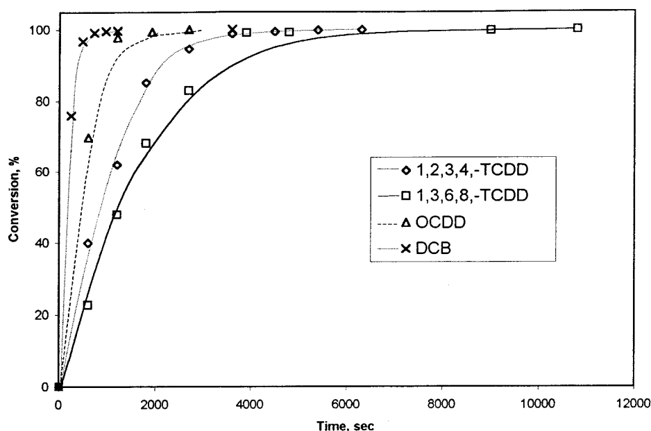
FIGURE 1. Disappearance of 1,2,3,4-TCDD, 1,3,6,8-TCDD, OCDD, and DCB during photolysis at 254 nm.
