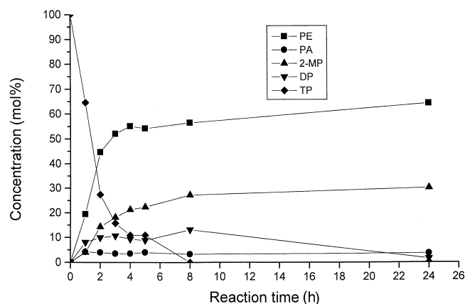
FIG. 1. Time course of the alcoholysis of tripalmitin with lipase from Rhizopus delemar immobilized on Celite. PE, palmitic acid ethyl ester; PA, palmitic acid; 2-MP, 2-monopalmitin; DP, dipalmitin; TP, tripalmitin; (mol%), mol of fatty acyl groups.
