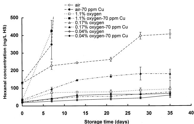
FIG. 5. Hexanal concentration [(ng/L) in the headspace (HS)] of the samples without and with 70 ppm copper in air, in 1.1% \text{O}_2 , in 0.17% \text{O}_2 , and in 0.04% \text{O}_2 . Error bars indicate standard deviations from three measurements.
