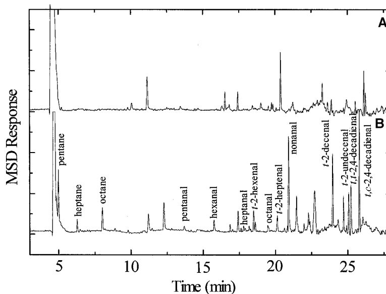
FIG. 2. Chromatographic profiles of compounds adsorbed by SPME, (A) before and (B) after microwave treatment.
