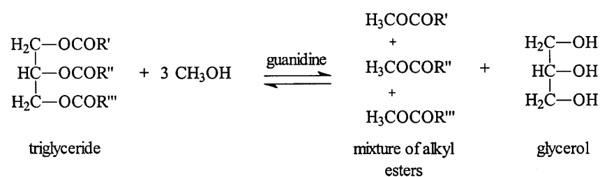
FIG. 2. Transesterification of vegetable oils.
