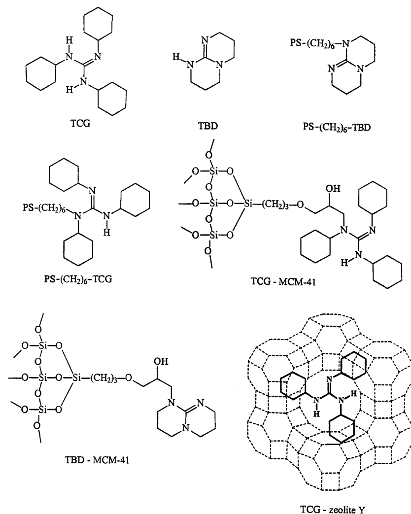
FIG. 1. Graphical representation of immobilized guanidines. TBD, 1,5,7-triazabicyclo [4.4.0]dec-5-ene; TCG, tricyclohexylguanidine; PS, polystyrene; MCM, a mesoporous ordered silica with channel diameters of 20–100 Å, prepared in the presence of surfactants as template agents.
