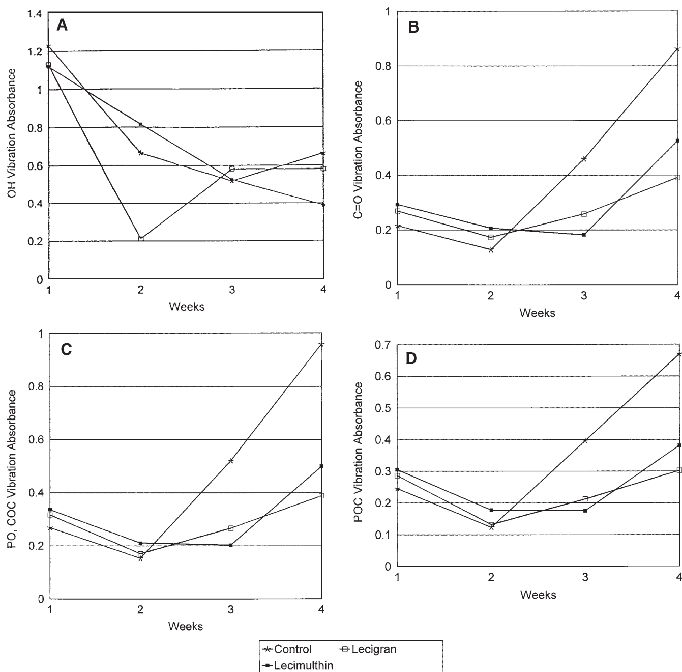
FIG. 2. The average FTIR absorbances of 4% Lecigran, 4% Lecimulthin, and control emulsions for the major vibration peaks from week 1 through week 4. (A) OH peak at 3348 cm -1 ; (B) C=O peak at 1741 cm -1 ; (C) PO and C–O–C peaks at 1157 cm -1 ; and (D) P–O–C peak at 1101 cm -1 . One hundred scans were co-added at a resolution of 4 cm -1 . See Figure 1 for abbreviation.
