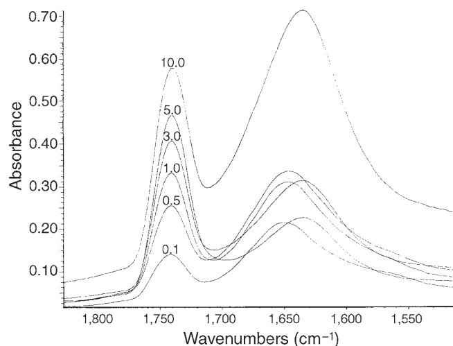
FIG. 5. The FTIR spectra of 4% Lecigran emulsions with 50 \mu\text{L} of 0.1, 0.5, 1.0, 3.0, 5.0, and 10.0 mg/mL of MgCl_2 with each 100 mL of emulsion. One hundred scans were co-added at a resolution of 4\text{ cm}^{-1} . (y axis is not to scale). See Figure 1 for abbreviations.
