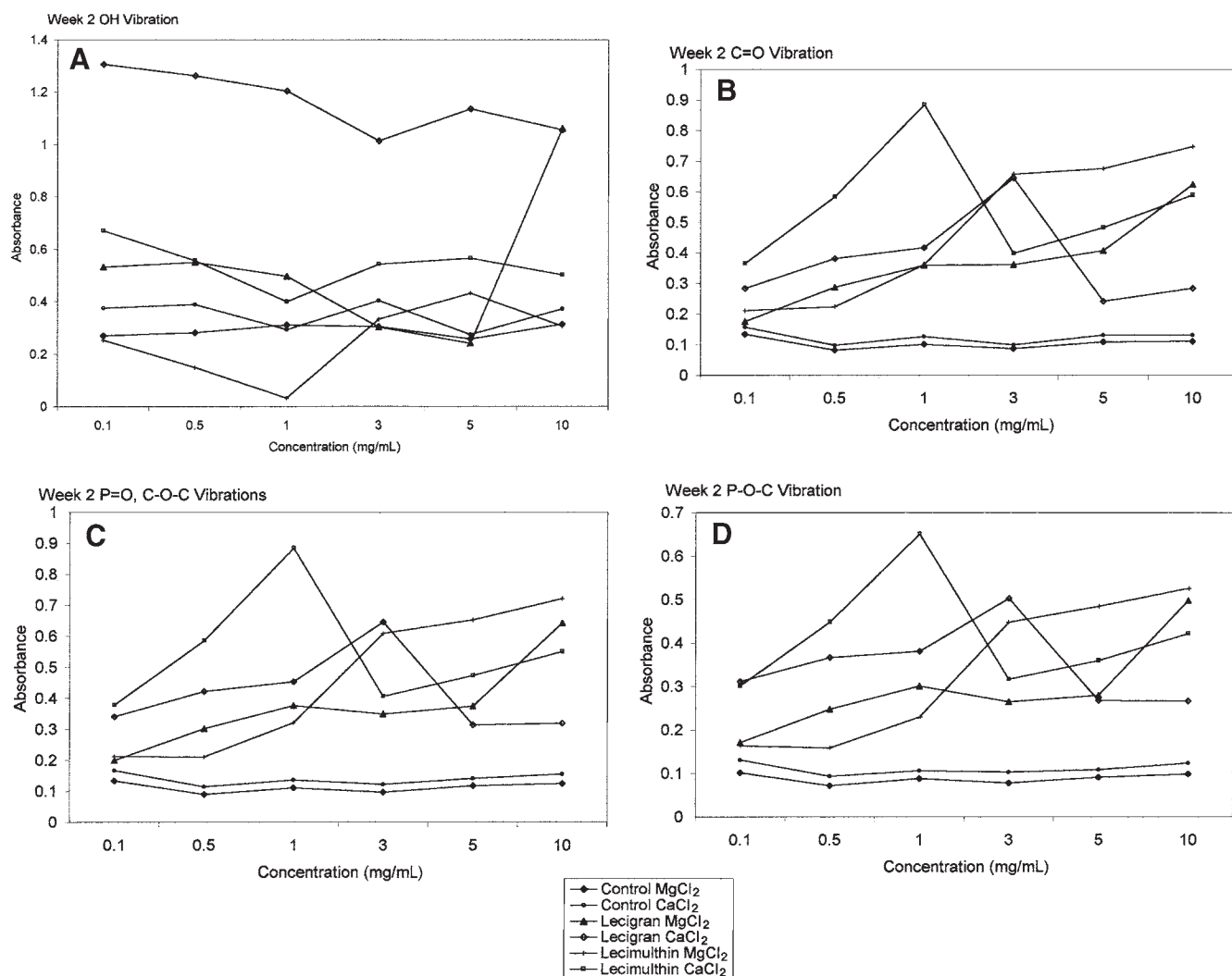
FIG. 4. The effect of addition of MgCl_2 and CaCl_2 on 4% Lecigran and 4% Lecimulthin and control emulsions for week 2. (A) OH peak at 3348\text{ cm}^{-1} ; (B) C=O peak at 1741\text{ cm}^{-1} ; (C) PO and C-O-C peaks at 1157\text{ cm}^{-1} ; and (D) P-O-C peak at 1101\text{ cm}^{-1} . One hundred scans were co-added at a resolution of 4\text{ cm}^{-1} .
