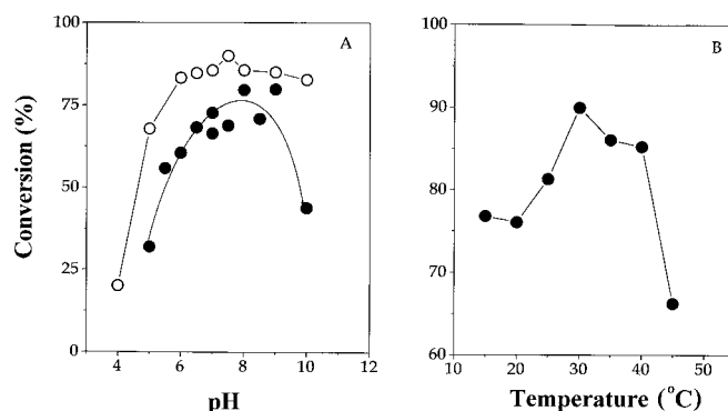
FIG. 3. pH and temperature dependence of esterification catalyzed by lipase in foams. (A) Oleyl oleate (○) and dodecyl oleate (●) formation were studied at various pH values at room temperature. Between pH 4–7 acetate buffer was used, and Tris-HCl buffer was used between pH 7–10. Comparison of esterification at overlapping pH values in the two buffers suggested that there were no buffer-specific effects. (B) Temperature dependence of dodecyl oleate formation in foams by lipase studied at pH 7.2. The activation energy of dodecyl oleate formation was calculated to be 24.4 kJ/mol.
