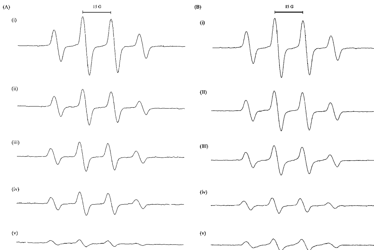
Figure 5. ESR spectra of the scavenging activity of (A) caffeic acid (I) and (B) quercetin 3-O-rutinoside (II) against hydroxyl radicals. (A) (i) control, (ii) 1 \mu M, (iii) 2 \mu M, (iv) 5 \mu M and (v) 7 \mu M; (B) (i) control, (ii) 5 \mu M, (iii) 7 \mu M, (iv) 10 \mu M and (v) 15 \mu M.
