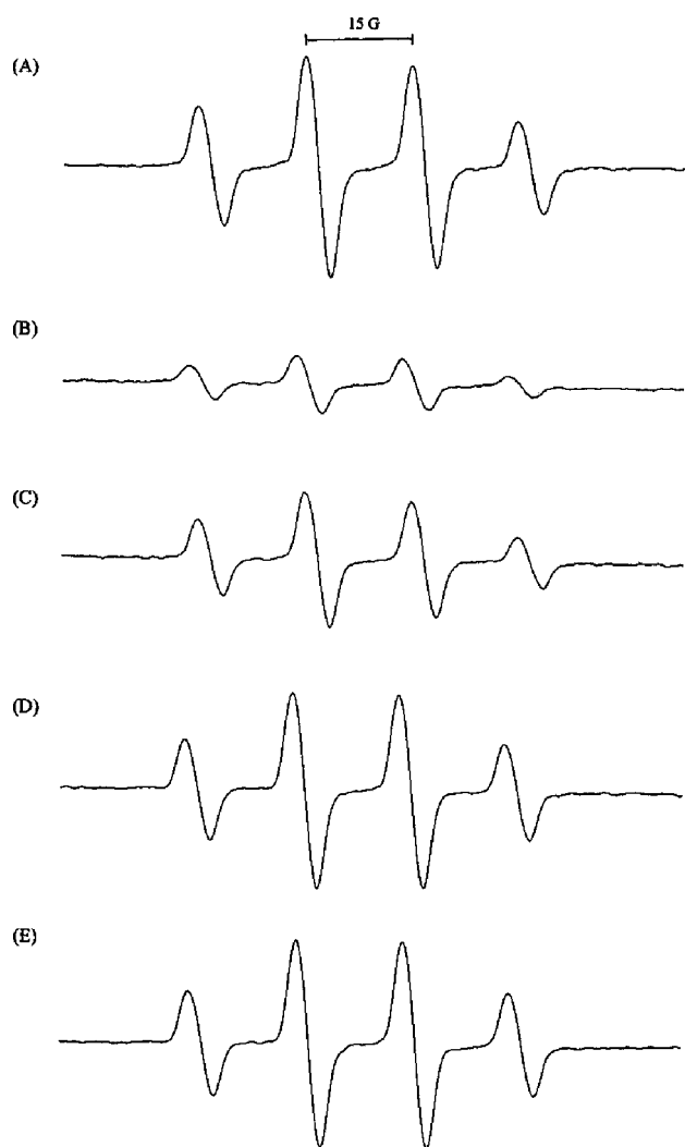
Figure 4. ESR spectra of the scavenging activity of the isolated constituents at 5 \mu M against hydroxyl radicals. (A) Control, (B) caffeic acid ( I ), (C) quercetin 3- O -rutinoside ( II ), (D) kaempferol 3- O -rutinoside ( III ), and (E) kaempferol 3- O -robinobioside ( IV ).
