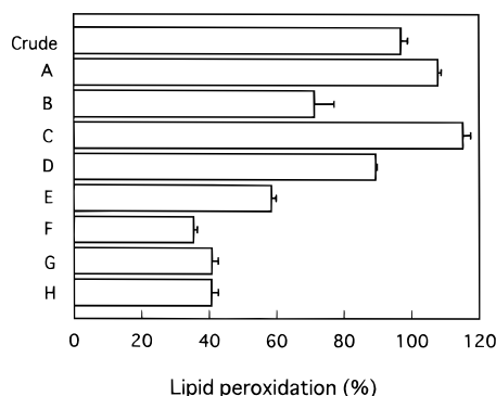
Figure 2. Rate of lipid peroxidation in the presence of the fractions ( 4.2 \times 10^{-3}\% w/v) separated by Sephadex LH-20 column chromatography. Data are mean \pm SE of three experiments. The crude extract was used as a reference.
