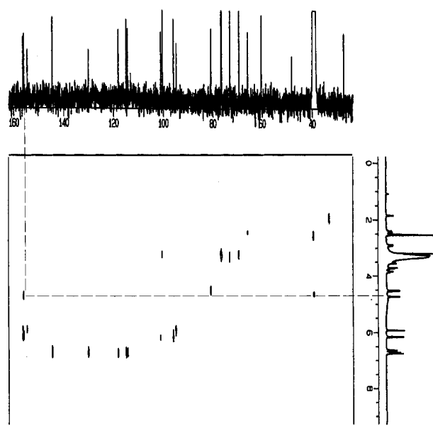
Figure 6. Heteronuclear long-range correlations observed by COLOC experiment in compound F 1 . DMSO- d 6 was used as the solvent.
