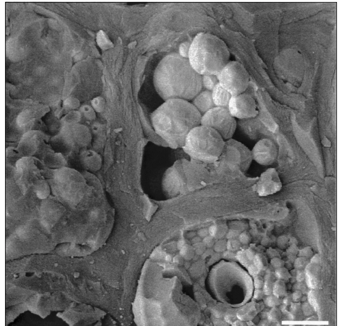
Fig. 7a—Cryo-SEM micrograph of a roasted coffee bean intruded with mercury during porosimetric analysis. Scale bar = 10 μm.
