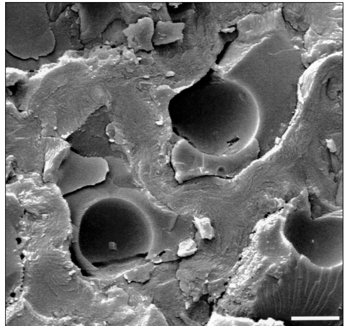
Fig. 3—Cryo-SEM micrograph of cells in green coffee beans. Scale bar = 10 \mu\text{m} .
