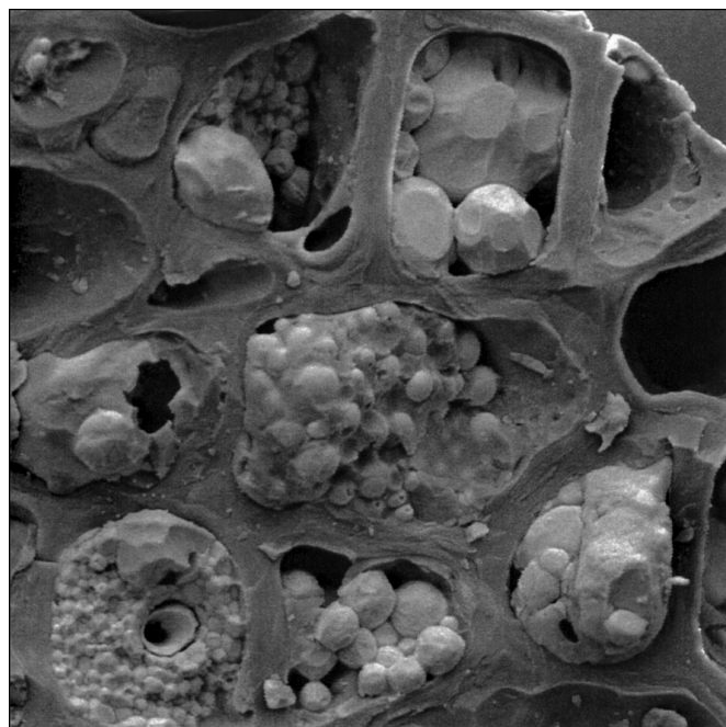
Fig. 6—Cryo-SEM micrograph of cells in a roasted bean intruded with mercury during porosimetric analysis. Integer cell wall structure with mercury-filled cell lumina. Image width = 137 μm.
