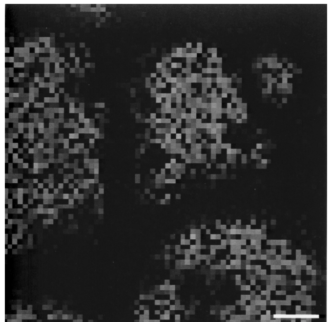
Fig. 7b—Mercury mapping obtained by X-ray microanalysis of a roasted coffee bean intruded with mercury (identical bean sample and sector as in 7a). Scale bar = 10 μm.
