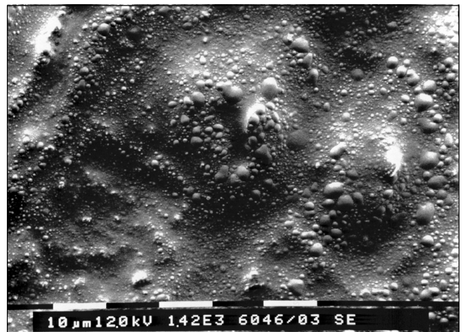
Fig. 10 —Cryo-SEM micrograph of the surface of a high-temperature roasted bean after 1 d of storage. Numerous very small oil droplets covering the surface show the beginning oil migration process and indicate the presence of an extensive network of micropores.
