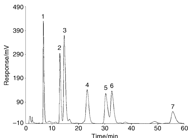
Fig. 1 HPLC separation at 22^\circ\text{C} of D,L-selenocystine, D,L-selenomethionine and D,L-selenoethionine enantiomers using UV absorbance detection at 200 \text{ nm} with 20 \mu\text{L} injection of a 1000 \mu\text{g mL}^{-1} standard. Mobile phase, 0.1 \text{ M HClO}_4 (pH 1), 0.5 \text{ mL min}^{-1} for 35 min then increased to 1.0 \text{ mL min}^{-1} . Peaks: 1 = L-selenocystine; 2 = L-selenomethionine; 3 = meso-selenocystine; 4 = D-selenocystine; 5 = D-selenomethionine; 6 = L-selenoethionine; and 7 = D-selenoethionine.
