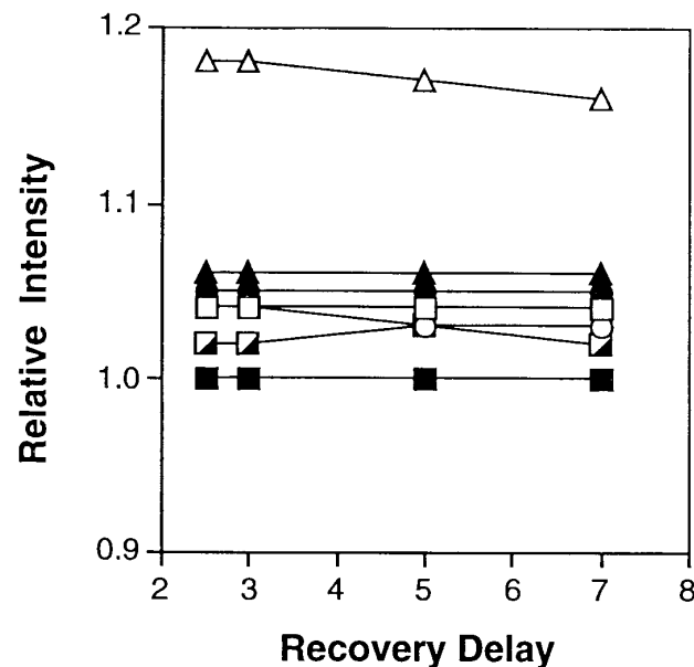
FIG. 3. Effect of recovery delay on the quantitativeness of the NMR spectrum. See Figure 1 for abbreviation. Relative intensity = (area of one peak)/(area of glyceryl group/4): \square , olefin; \circ , \alpha -methylene; \triangle , \beta -methylene; \blacksquare , methyl; \blacksquare , glycerin; \bullet , allyl; \blacktriangle , methylene.
