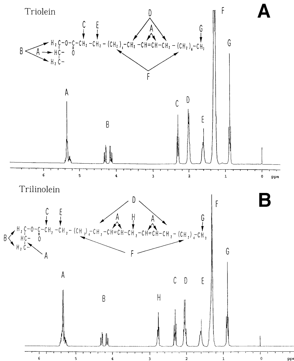
FIG. 1. 1 H nuclear magnetic resonance (NMR) spectrum of triolein (A) and trilinolein (B).
