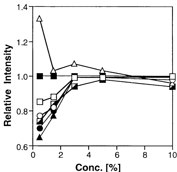
FIG. 2. Effect of sample concentration on the quantitativeness of the NMR spectrum. See Figure 1 for abbreviation. Relative intensity = (area of one peak)/(area of glyceryl group/4): \square , olefin; \circ , \alpha -methylene; \triangle , \beta -methylene; \blacksquare , methyl; \blacksquare , glycerin; \bullet , allyl; \blacktriangle , methylene.
