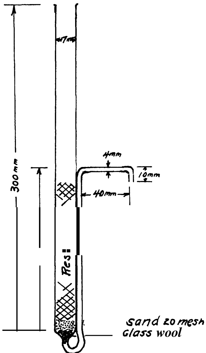
FIG. 4.-Adsorption tube.
