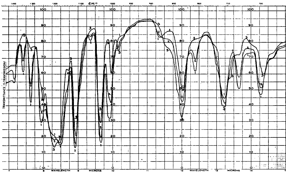
FIG. 10.—FD&C Orange No. 1, D&C Orange No. 4, and Mixture. Conc.: 10.0 mg./ml. Suspended in CS 2 Cells: 0.5 mm. Curve 1—FD&C Orange No. 1 Curve 2—Mixture \left\{ \begin{array}{l} 60\% \text{ FD\&C Orange No. 1} \\ 40\% \text{ D\&C Orange No. 4} \end{array} \right. Curve 3—D&C Orange No. 4
