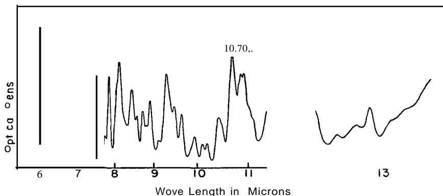
FIG. I.-The infrared absorption spectrum of methyltestosterone 10 mg/ml OS. 1.0 mm cell.
