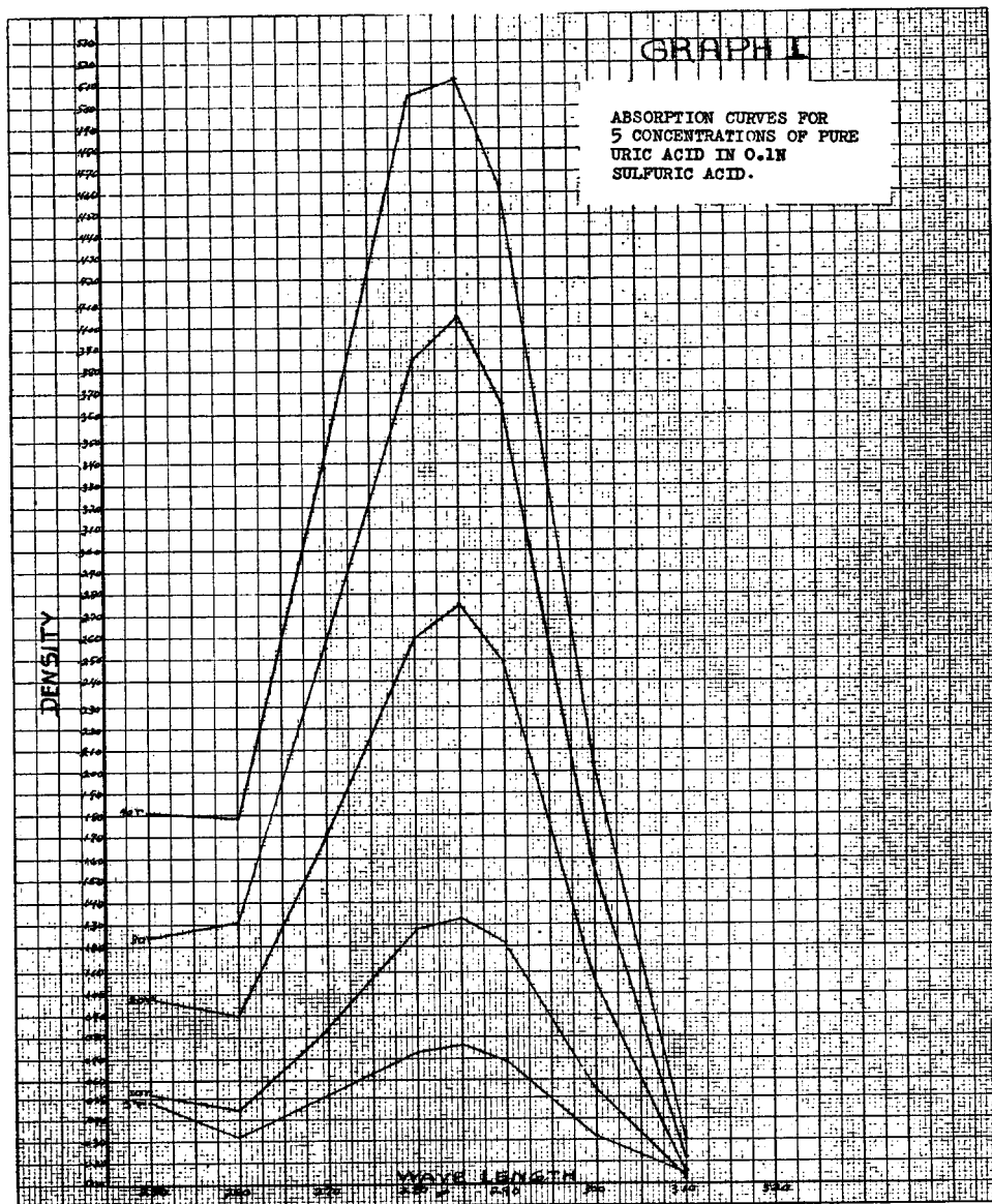
GRAPH I.—Absorption curves for 5 concentrations of pure uric acid in 0.1 N sulfuric acid.
