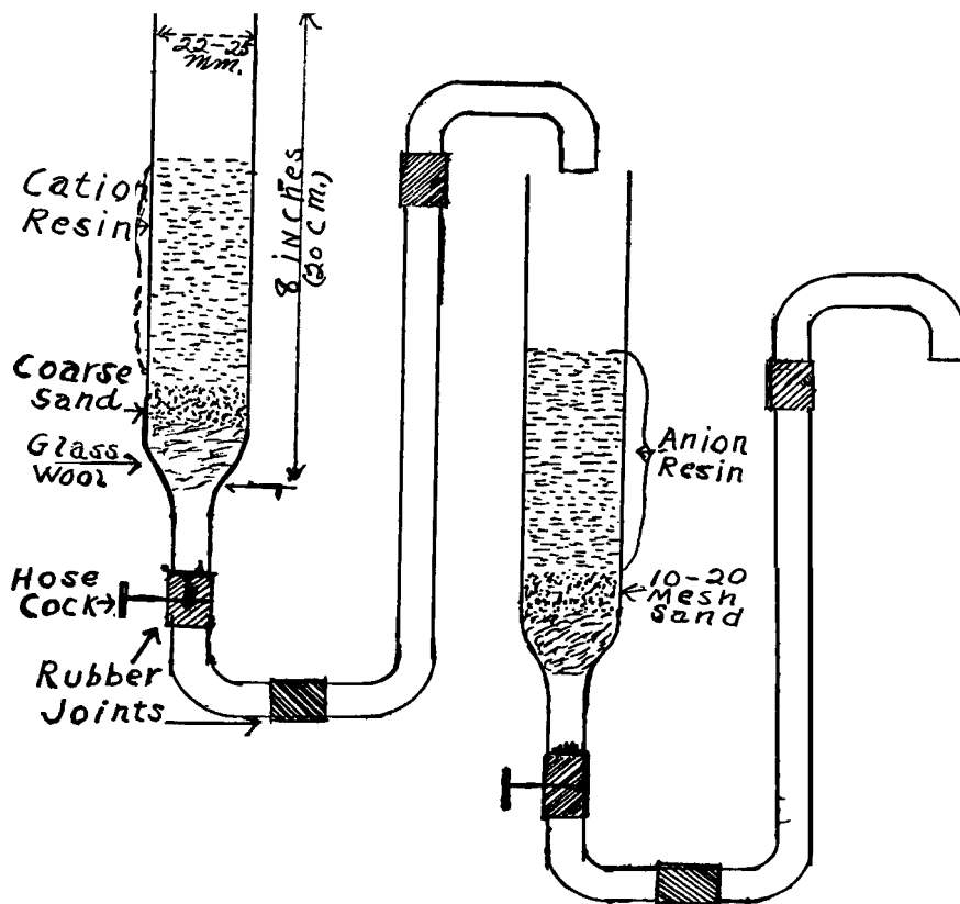
FIG. 2.-Ion exchange tubes
