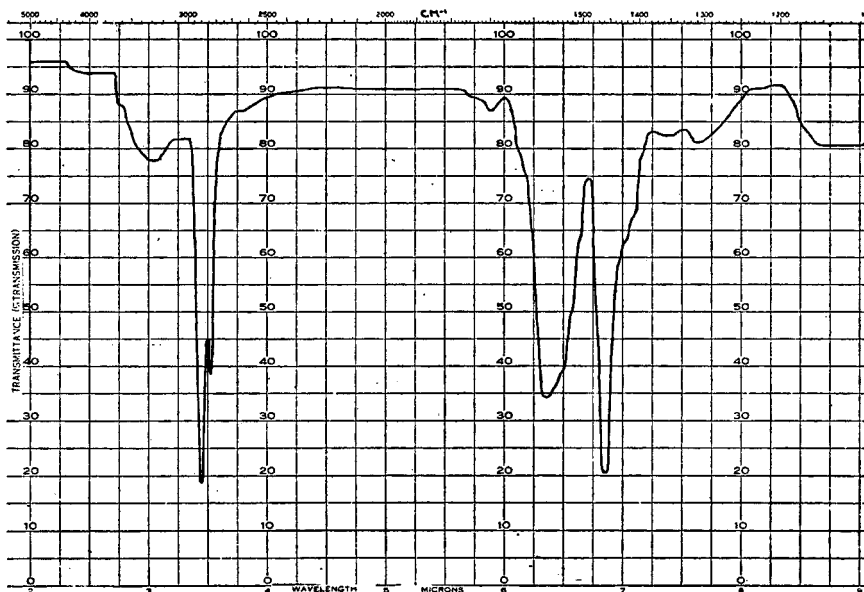
FIG. 2.—Aluminum Stearate Conc: 10.0 mg./ml. Solvent: Carbon tetrachloride Cells: 0.5 mm.
