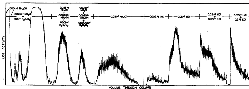
Fig. 3. Separation of ^{32}\text{P} -labeled compounds from Wintex barley by the method of KHYM AND COHN 3 .
