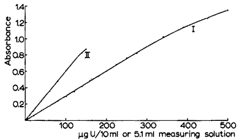
Fig. 4. Calibration curves.
