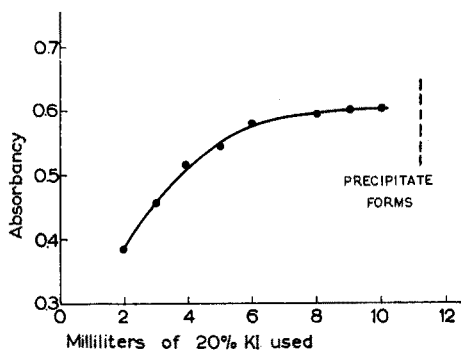
Fig. 6. Effect of amount of KI used on solution absorbance. 7.7 p.p.m. Ir used in the test solutions. Absorbance measured at 446 m\mu .
