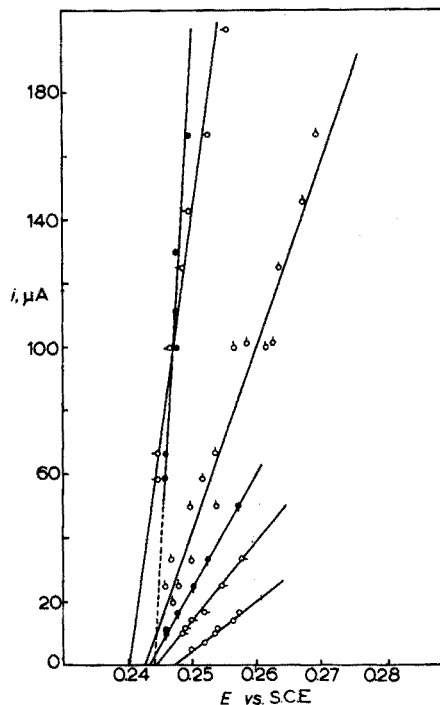
Fig. 3. Variation of E_{1/2} with i_0 and ferrocyanide concentration. KCl concentration constant at 1.5 M. Ferrocyanide concentration 2 (○), 4 (◊), 6 (●), 10 (◊), 30 (◻), and 40 (●) \cdot 10^{-4} M.
