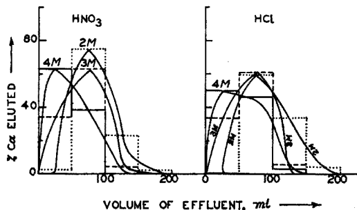
Fig. 1. Cation-exchange behavior of calcium with HCl and HNO 3 as eluents.
