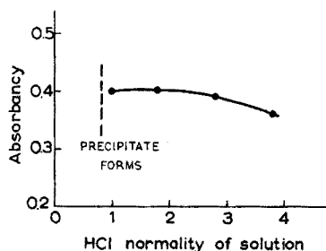
Fig. 5. Variation of solution absorbancy (446 m\mu ) with concentration of hydrochloric acid. 5.5 p.p.m. Ir used in test solutions.
