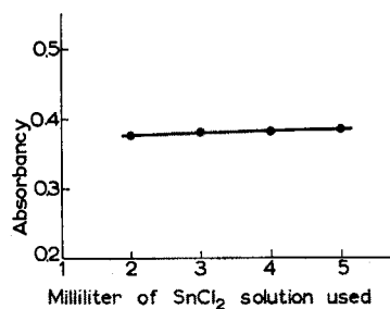
Fig. 7. Effect of amount of SnCl 2 used on solution absorbance. 5.5 p.p.m. Ir used in the test solutions. Absorbance measured at 446 m\mu .
