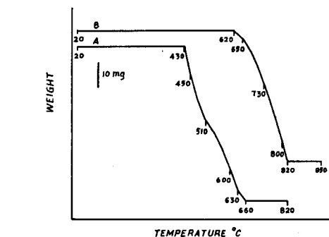
Fig. 3. Thermal decomposition curves of selenides precipitated by sodium selenide reagent. A, antimony pentaselenide; B, silver selenide.
