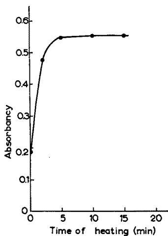
Fig. 1. Effect of time of heating on the conversion of hexachloroiridite to hexaiodoiridite. 7.7 p.p.m. Ir used in the test solution. Absorbancy measured at 446 \text{ m}\mu .
