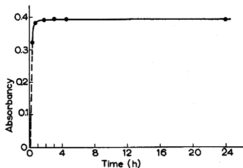
Fig. 2. Variation of solution absorbancy ( 446 \text{ m}\mu ) with time of color development at room temperature. 5.8 p.p.m. Ir used in the test solutions.
