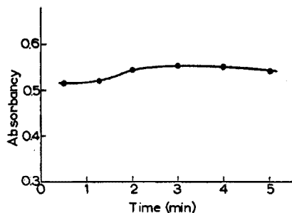
Fig. 3. Variation of solution absorbancy ( 446 \text{ m}\mu ) with time of heating in boiling water bath after the addition of stannous chloride solution and dilution to volume. 7.7 p.p.m. Ir used in the test solutions.
