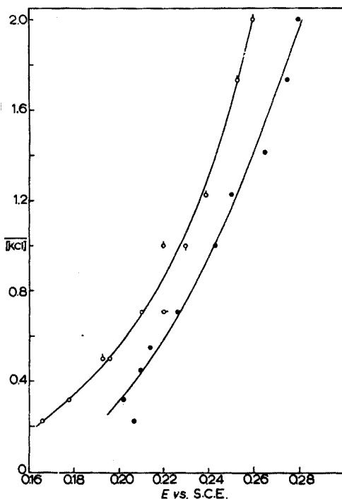
Fig. 2. Variation of E_{p/2} + 0.028 V with KCl concentration. (●) Experimental points, mean values; (○) Potentiometric data, Pt electrode 23 ; (◊) Potentiometric measurement, graphite electrode 20 ; (○) Formal potential, Pt electrode 21 ; (◊) Potentiometric data, Pt electrode 24 .
