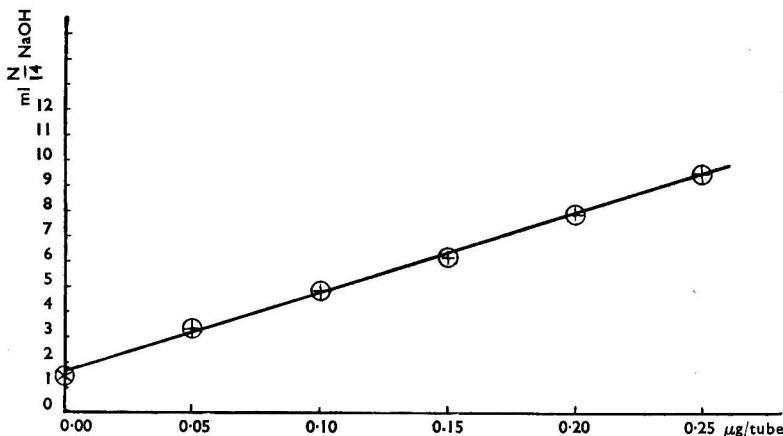
Fig. 2. Nicotinic Acid
