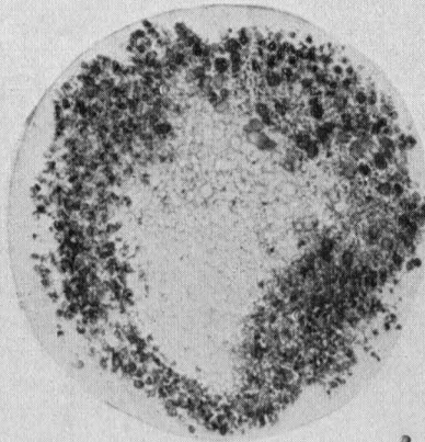
Plate I "Lead Prints" of leaded steel.
