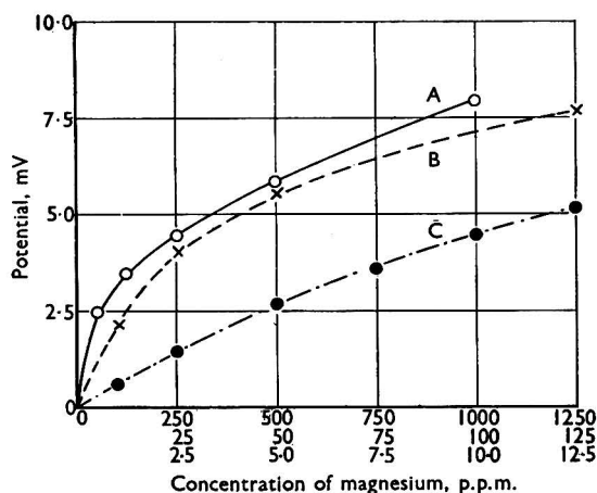
Fig. 3. Standard curves for magnesium (linear co-ordinates): curve A, 0 to 1000 p.p.m.; curve B, 0 to 125 p.p.m.; curve C, 0 to 12.5 p.p.m.
