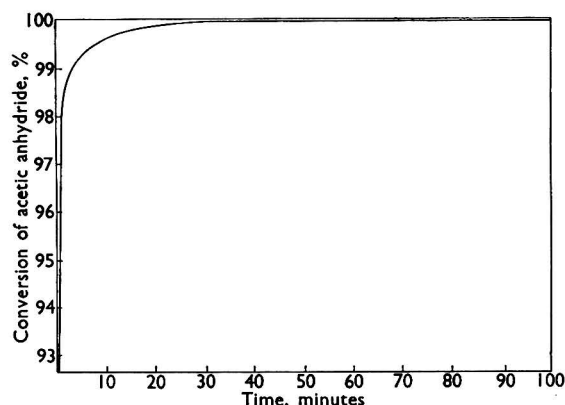
Fig. 3. Rate of reaction of acetic anhydride with excess of aniline at 20°C
