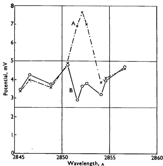
Fig. 2. Emission readings in the region of 2852 Å: A, 10 p.p.m. of magnesium; B, background. Approximate readings for wavelength correction. Slit width, 0.03 mm
