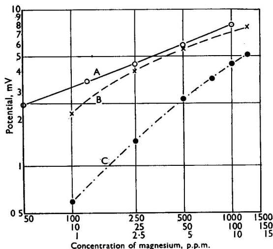
Fig. 4. Standard curves for magnesium (logarithmic co-ordinates): curve A, 50 to 1000 p.p.m.; curve B, 10 to 125 p.p.m.; curve C, 1 to 12.5 p.p.m.
