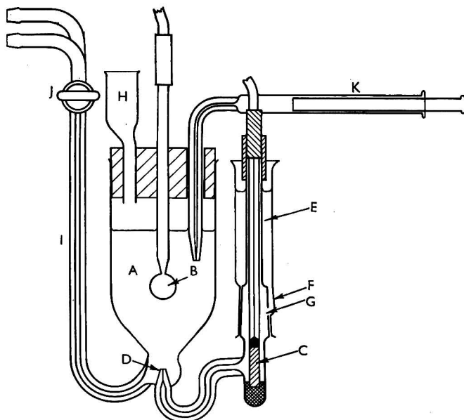
Fig. 4. Titration assembly: A, titration cell; B, glass electrode; C, saturated-calomel half-cell; D, hair capillary; E, reservoir; F, ridge; G, hole; H, funnel; I, tube; J, three-way tap; K, glass syringe
