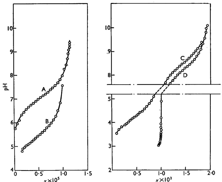
Fig. 3. pH- x curves: curve A, 2:4:5-trichlorophenol; curve B, 2:3:4:6-tetrachlorophenol; curve C, quinine; curve D, brucine
