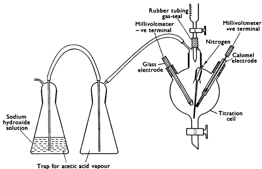
Fig. 1. Potentiometric-titration apparatus, with a trap for acetic acid vapour
