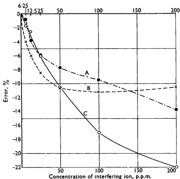
Fig. 5. Error in the determination of 10.00 p.p.m. of magnesium in the presence of interfering ions: curve A, sulphate sulphur; curve B, phosphate phosphorus; curve C, aluminium
