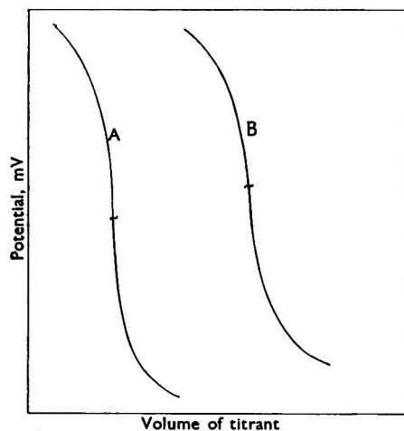
Fig. 2. Standardisation curves: curve A, perchloric acid against sodium carbonate; curve B, aniline against perchloric acid
