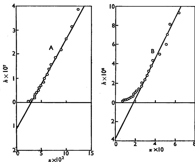
Fig. 7. h - z curves derived from Fig. 6
