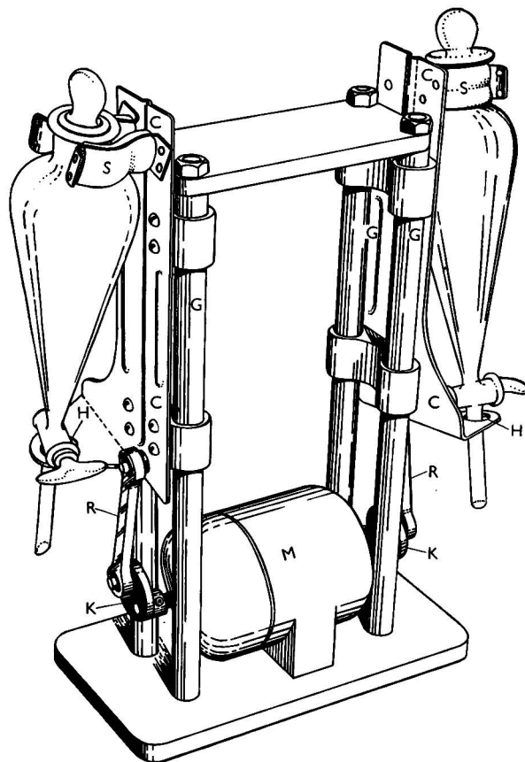
Fig. 1. Mechanical shaker
