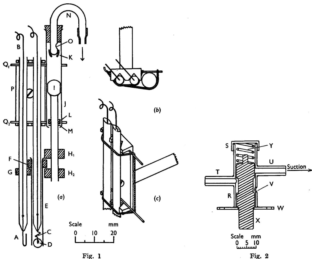
Fig. 1. Differential electrode system: (a), front view (sectional); (b), diagrammatic top view; (c), method of retaining electrode tubes
