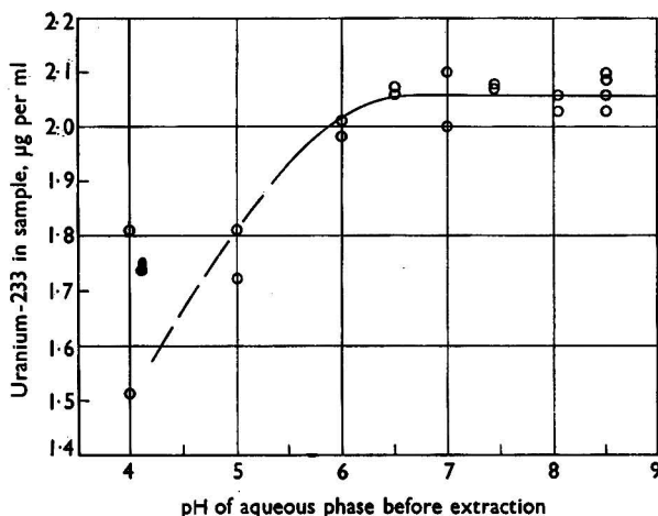
Fig. 1. Extraction of uranium-233 from thorium nitrate solutions by means of a 2.5 per cent. solution of oxine in hexone (0.17 M ) as a function of pH. The concentrations of uranium and thorium were 10^{-5} M and 1.3 \times 10^{-3} M , respectively
