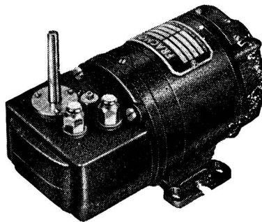
Illus. : Type 334C40 Geared Motor, with A.C. and D.C. inter- changeable frames. 1-20 r.p.m. Torque: 20-10 lbs./ins.
