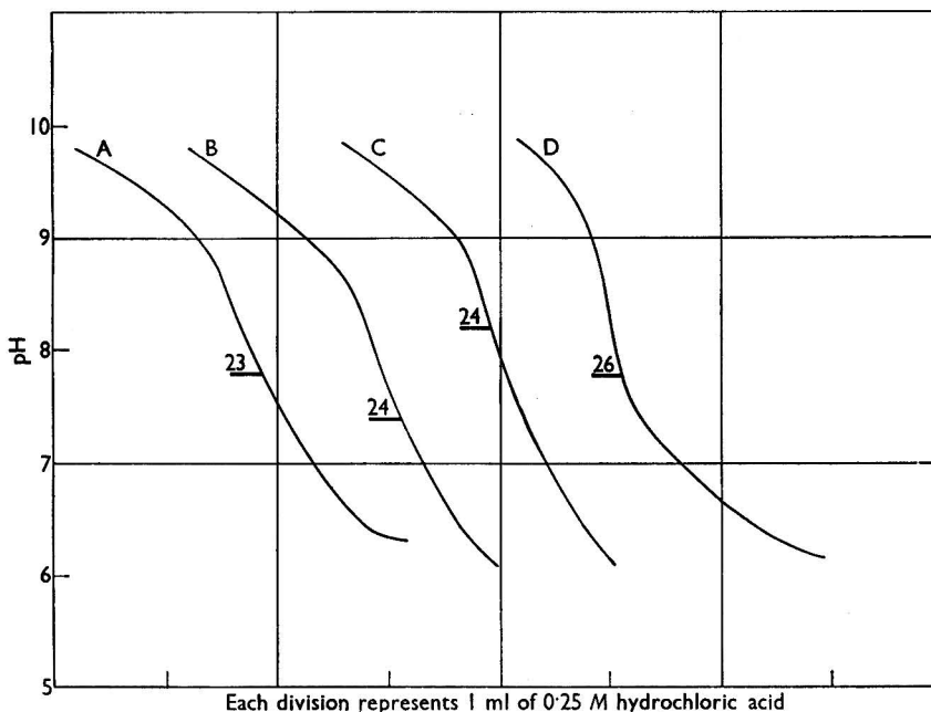
Fig. 3. Titration of unused 0.25 M sodium hydroxide after addition of: curve A, (\text{NH}_4)_3[\text{P}(\text{Mo}_3\text{O}_{10})_4] ; curve B, "synthetic" (\text{NH}_4)_2\text{H}[\text{P}(\text{Mo}_3\text{O}_{10})_4] ; curve C, (\text{NH}_4)_2\text{H}[\text{P}(\text{Mo}_3\text{O}_{10})_4]\cdot\text{H}_2\text{O} ; curve D, (\text{NH}_4)_2\text{H}[\text{P}(\text{Mo}_3\text{O}_{10})_4]\cdot\text{H}_2\text{O} , after treatment with formaldehyde. The theoretical end-points are shown on each curve
