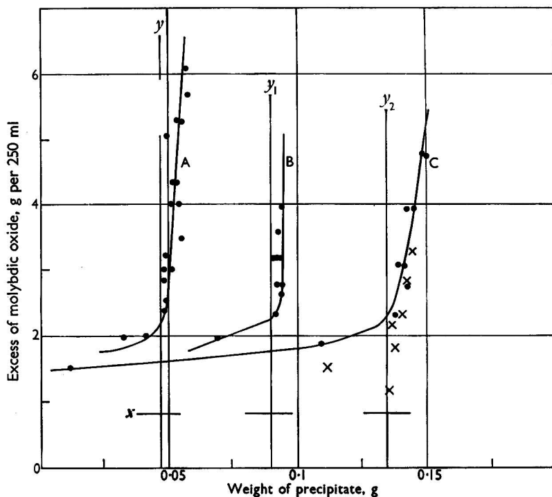
Fig. 2. Determination of phosphorus in various steels: curve A, 3 g of a steel containing 0.028 per cent. of phosphorus at 60° C; curve B, 2 g of a steel containing 0.076 per cent. of phosphorus at 40° C; curve C, 3 g of a steel containing 0.076 per cent. of phosphorus at 60° C. Points marked X represent an experiment in which nitrate ions were replaced by perchlorate ions. Ordinates y , y_1 and y_2 represent the theoretical weight of precipitate; the abscissa x represents the limiting conditions when potassium dihydrogen phosphate is used in place of the steel
