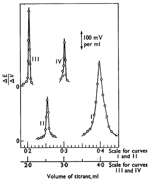
Fig. 3. Differential titrations: curve I, 2.0 ml of 0.002 N hydrochloric acid with 0.01 N sodium hydroxide; curve II, 2.55 ml of 0.1 N acetic acid with N sodium hydroxide; curve III, 2.0 ml of 0.1 N sodium acetate with 0.098 N perchloric acid, both in glacial acetic acid solution; curve IV, 3.0 ml of 0.1 N antimony trichloride with 0.1 N bromine, both in glacial acetic acid solution
