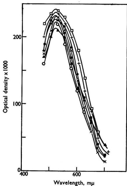
Fig. 2. Absorption curves for ethyl esters of fatty acids of different chain lengths. Concentration of esters, 2.5 \times 10^{-4} M : □, oleate; ●, stearate; ○, palmitate; +, laurate; ×, octanoate; ▲, butyrate; ■, acetate
