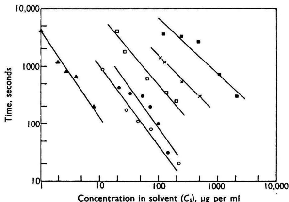
Fig. 2. Time required for extraction of minimum detectable amount of caffeine from various solvents: \blacktriangle , cyclohexane; \circ chloroform-cyclohexane mixture (1 + 5 v/v); \bullet , carbon disulphide; \square , chloroform-cyclohexane mixture (1 + 1 v/v); \times , chloroform; \blacksquare , ethylene dichloride
