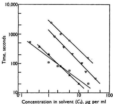
Fig. 3. Time required for extraction of minimum detectable amount of cocaine from various solvents: \blacktriangle , cyclohexane; \nabla , chloroform; \circ , nitrobenzene; \square , ethylene dichloride
