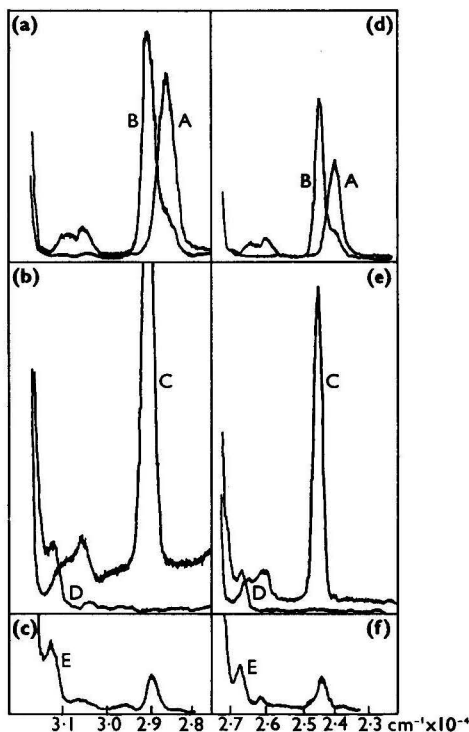
Fig. 1. Recordings of Raman bands excited by (a), (b) and (c), 313\text{-m}\mu light, (d), (e) and (f), 365\text{-m}\mu light: curve A, water; curve B, ethanol; curve C, cyclohexane ; curve D, carbon tetrachloride; curve E, chloroform
