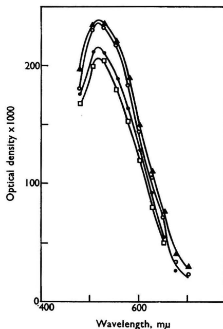
Fig. 3. Absorption curves for various acetates. Concentration of esters, 2.5 \times 10^{-4} M : ●, methyl acetate; ▲, ethyl acetate; ○, glyceryl acetate; □, cholesteryl acetate
