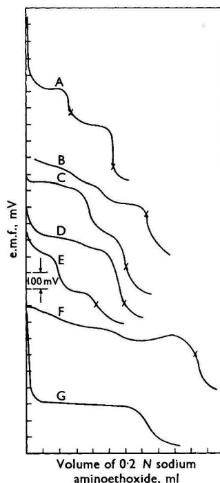
Fig. 2. Typical titration curves for phenolic compounds: curve A, 1:3-dihydroxynaphthalene; curve B, 1:3-dihydroxynaphthalene plus 2:6-xyleneol; curve C, 1:5-dihydroxynaphthalene plus 2:6-xyleneol; curve D, pyrogallol plus 2:6-xyleneol; curve E, 2-hydroxy-1:4-naphthaquinone plus 2:6-xyleneol; curve F, a mixture of 2:6 xyleneol, catechol, 1:5-dihydroxynaphthalene and 1:8-dihydroxyanthraquinone; curve G, a tar acid-fraction. Theoretical end-points are indicated by crosses
