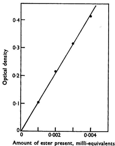
Fig. 1. Typical calibration graph for glyceryl trioleate
