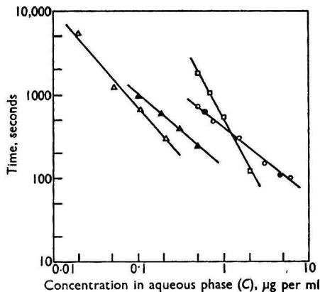
Fig. 4. Time required for two-stage extraction of minimum detectable amounts of nicotine and morphine from aqueous solutions: \triangle , nicotine in pH 8.0 buffer solution extracted with chloroform; \blacktriangle , nicotine in pH 6.5 buffer solution extracted with chloroform; \square , nicotine in pH 8.0 buffer solution extracted with light petroleum, boiling range 100° to 110° C; \circ , morphine in pH 8.0 buffer solution extracted with chloroform; \bullet , morphine in pH 8.0 buffer solution extracted with chloroform-ethanol mixture (10 + 1 v/v)
