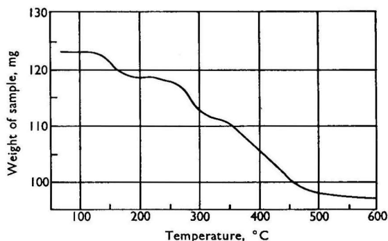
Fig. 1. Effect of heating a sample of tri- n -butylammonium tungstophosphate in a thermobalance
