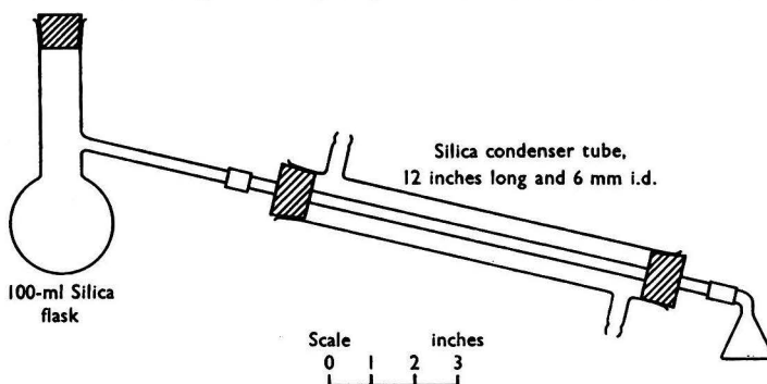
Fig. 1. Distillation apparatus
