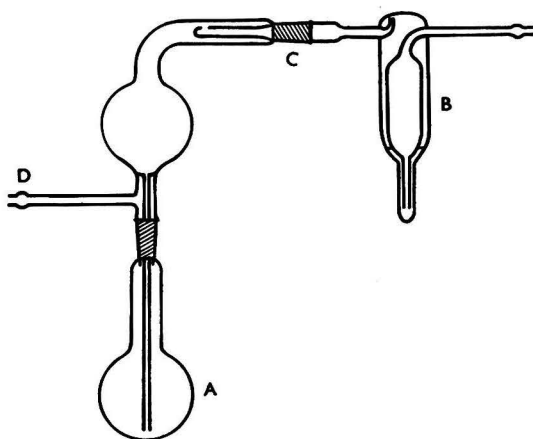
Fig. 2. Apparatus for preparing boron trifluoride - ether complex
