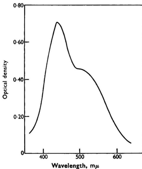
Fig. 1. Absorption spectrum of 2:4-dinitrophenylhydrazone in alkaline solution
