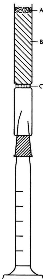
Fig. 3. Storage container for boron trifluoride - ether complex: A, glass wool; B, silica gel; C, sintered-glass disc
