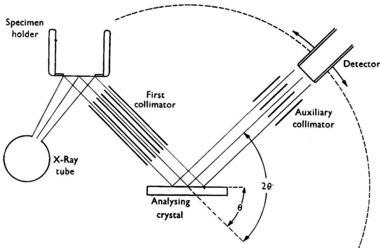
Fig. 5. Diagrammatic arrangement of the plane-crystal X-ray spectrograph
