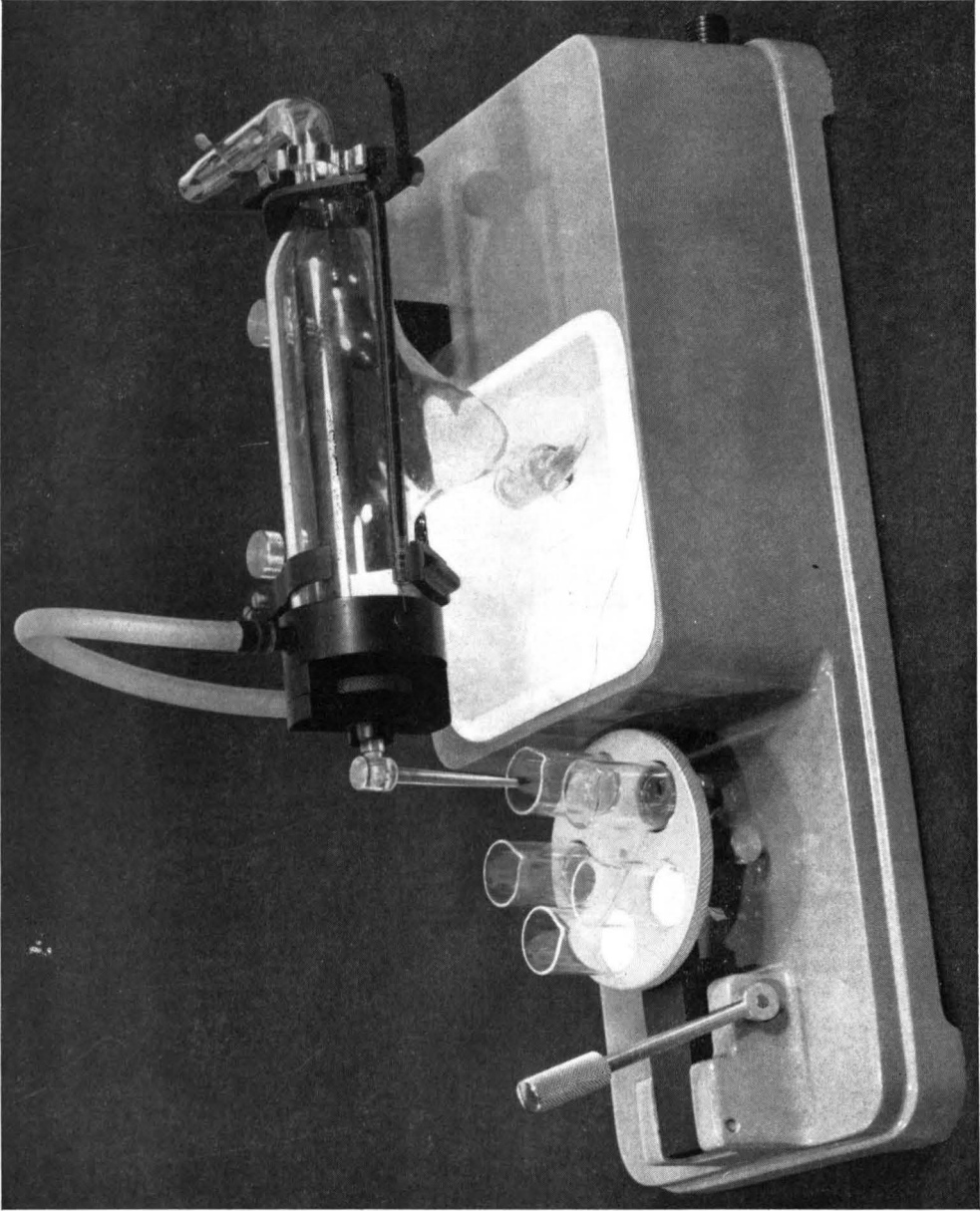
Fig. 1. Atomic-absorption attachment showing spray, spray chamber and sample beakers
