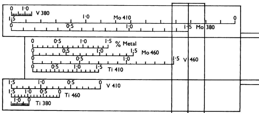
Fig. 1. Slide rule
