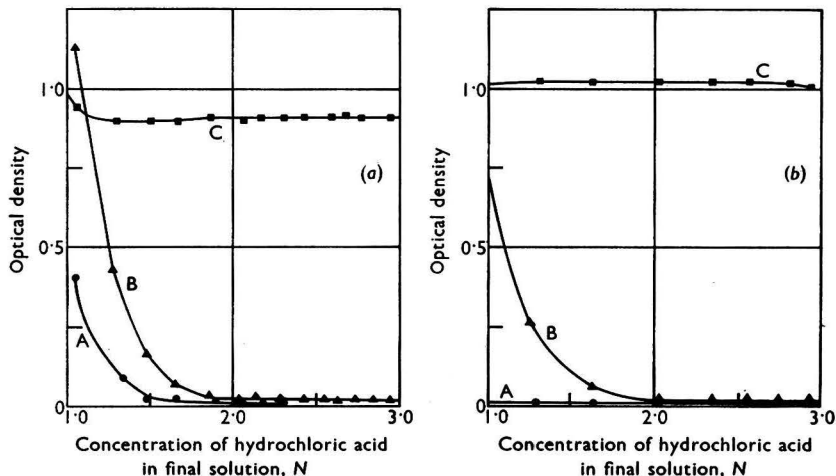
Fig. 2. Effect of acid concentration on reduction of ammonium molybdate, molybdophosphate and molybdosilicate (a) with no interval between increase in acidity and reduction, (b) with 10-minute interval: curve A, 50 ml of 1 per cent. w/v acidified ammonium molybdate solution and x ml of 50 per cent. v/v hydrochloric acid; curve B, 50 ml of 1 per cent. w/v acidified ammonium molybdophosphate solution, 20 ml of 0.0053 per cent. w/v potassium dihydrogen orthophosphate solution and x ml of 50 per cent. v/v hydrochloric acid; curve C, 50 ml of 1 per cent. w/v acidified ammonium molybdosilicate solution, 20 ml of 0.004 per cent. w/v silica solution and x ml of 50 per cent. v/v hydrochloric acid
