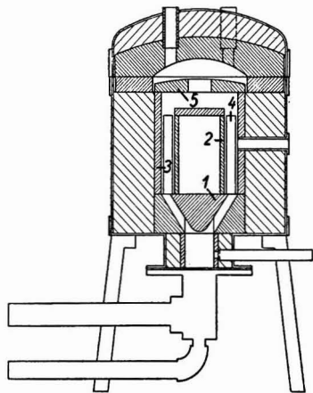
Degussa "Lilliput" Gas-heated Laboratory Furnace
