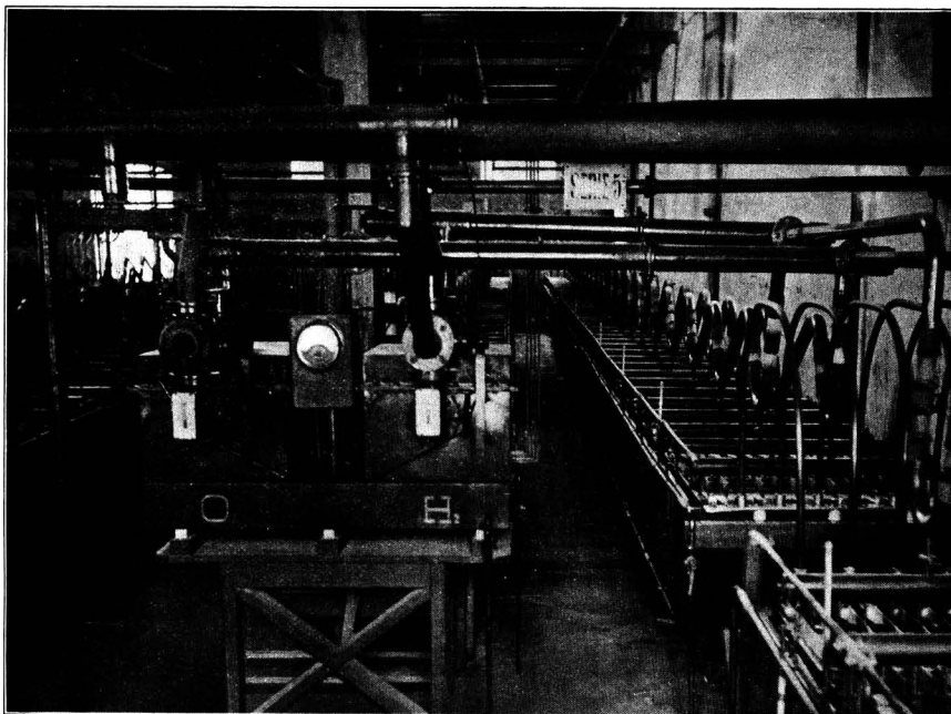
Extension to an Electrolytic Hydrogen Plant at Bussi, Italy, comprising 50 cells operating at 6,000 amperes
