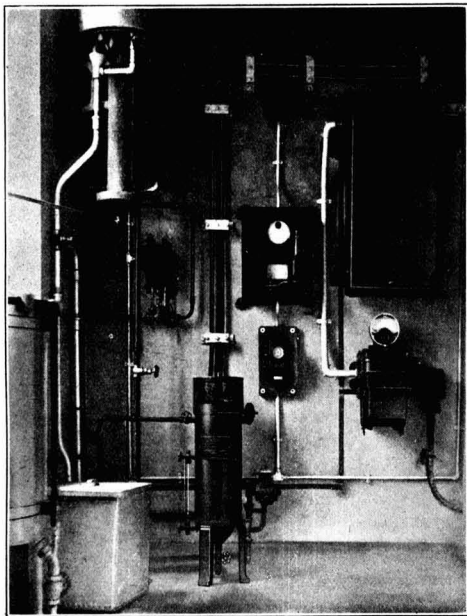
Electrode Boiler Installation for Distilled Water
