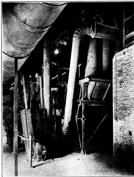
Typical Dust Exhausting Plant as designed by the Sturtevant Engineering Co., Ltd
