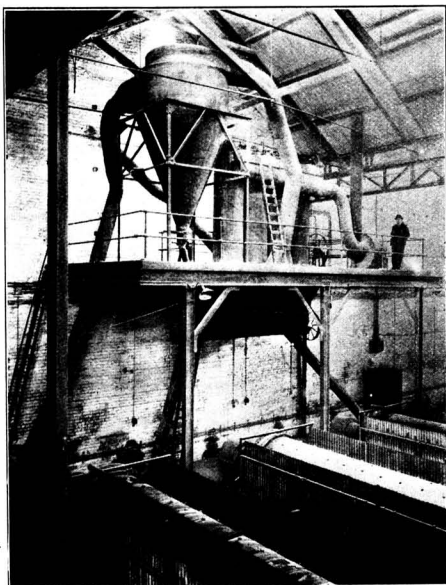
Typical Dust Exhausting Plant as designed by the Sturtevant Engineering Co., Ltd
