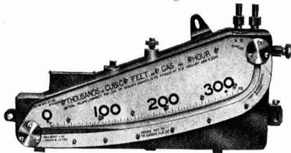
Fig. 3. Kent's Curved Tube Manometer
