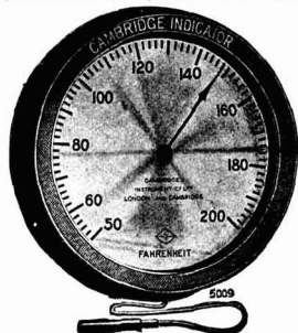
Indicating Mercury-in-Steel Thermometer (Cambridge Instrument Co.)
