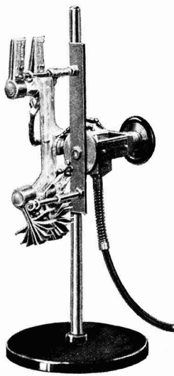
The U.V.S.A. Model Quartz Lamp for operation at any angle
