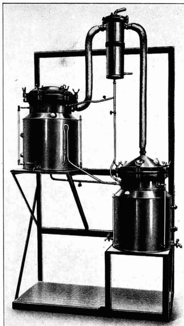
Improved Type of Soxhlet Extractor
