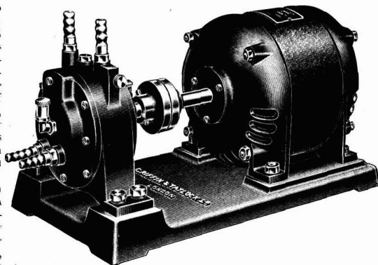
Laboratory Blower with Direct-coupled Motor.
