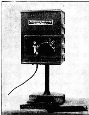
The Hanovia Analytical Quartz Lamp
