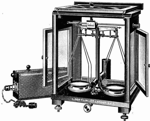
Prismatic Reflecting Aperiodic Balance No. 52P
