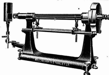
The Bellingham and Stanley Polarimeter
