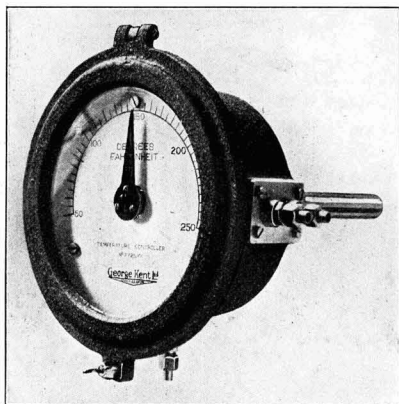
Fig. 1. Kent's Temperature Controller
