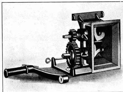
Mixing and Kneading Machine for Laboratory Use.
