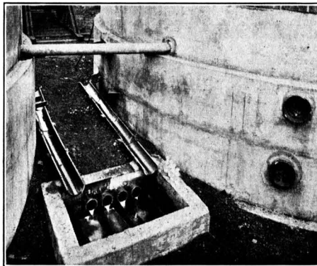
Arrangement of Effluent Outlets and Side Sampling Pipes on Filters at Beet Sugar Factory, Colwick, 1928-29
