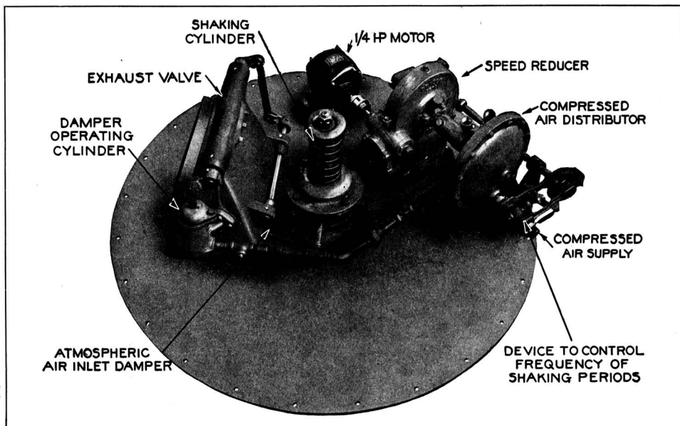
"Dracco" Dust Collecting System: Gear on Top Plate of Compartment
