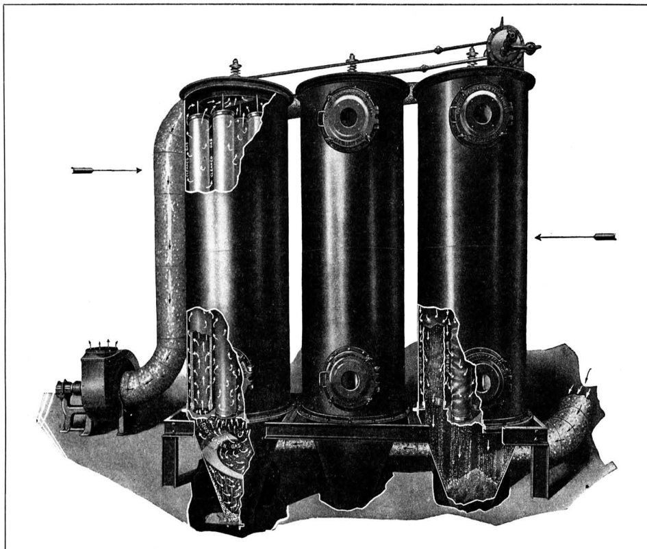
A Three Compartment "Dracco" Dust Collecting Unit
