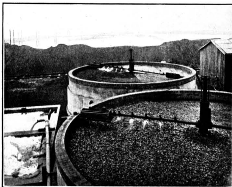
Filters of Experimental Purification Plant at Beet Sugar Factory, Colwick, 1928-29
