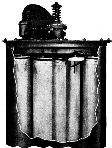
The Internal Supporting Arrangement for Bag Filters
