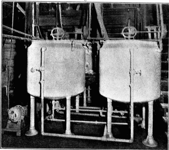
A battery of Pfaudler Mixers at the works of the Larrow-Suzuki Co., Rossford, dealing with liquids containing Hydrochloric Acid. These open type mixers, which are steam or brine jacketed, may also be used for evaporating, sulphoning, heating and cooling operations.
