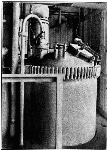
One of the standard Pfaudler Reaction Kettles, as installed at the works of the H. K. Mulford Co., Philadelphia, for Pharmaceutical Products, containing traces of Acid.
