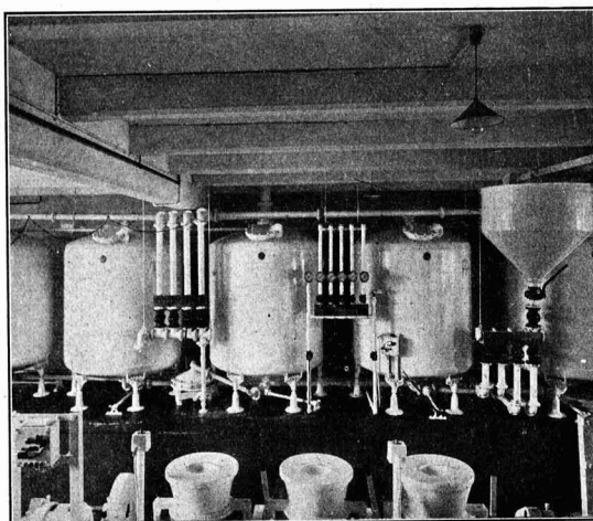
Pfaudler Glass Lined Equipment for Mixing and Storing Kolynos Dental Cream. (Enamelled Metal Products Corporation, 1933, Ltd.)
