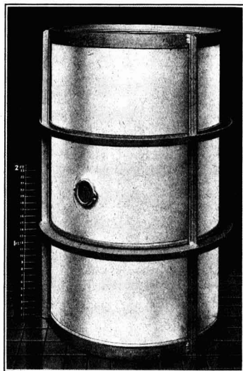
All-Welded Aluminium Drum (Aluminium Plant and Vessel Co., Ltd.).
