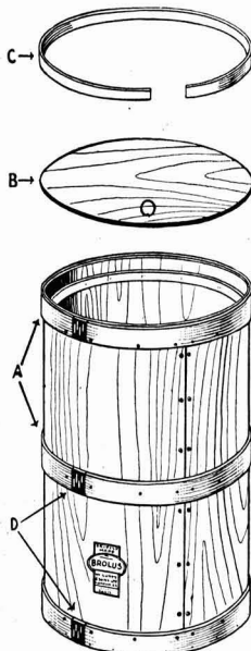
Brolus Plywood Barrel (W. Lusty and Sons, Ltd.).
