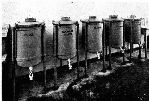
Pfaudler Glass Lined Equipment for Storage of Perfumery (Enamelled Metal Products Corporation, 1933, Ltd.).
