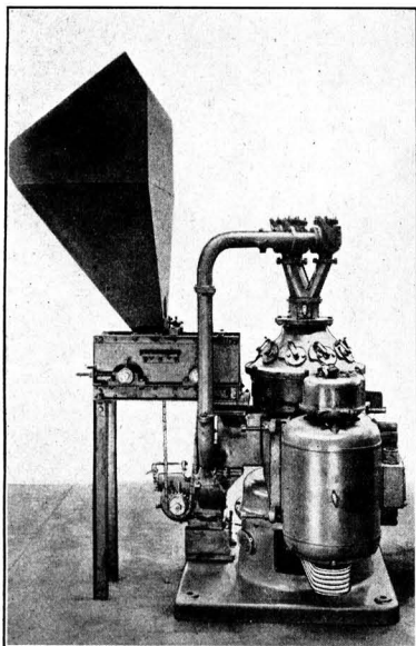
Left: A vertical V-Rope Drive is incorporated in this pulverised fuel firing unit.
