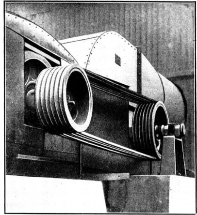
The V-Rope Drive has proved very efficient between the motor and the fan at this metallurgical plant.
