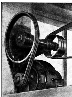
Left: In this reduction drive the centres of the motor pulley and countershaft pulley are almost at the minimum distance.
