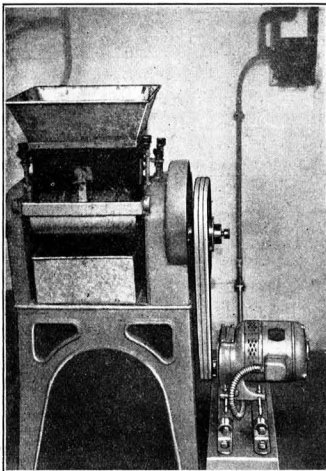
This machine is equipped with a geared motor and a V-Rope Drive, a speed reduction from 1425 to 120 r.p.m. being obtained.
