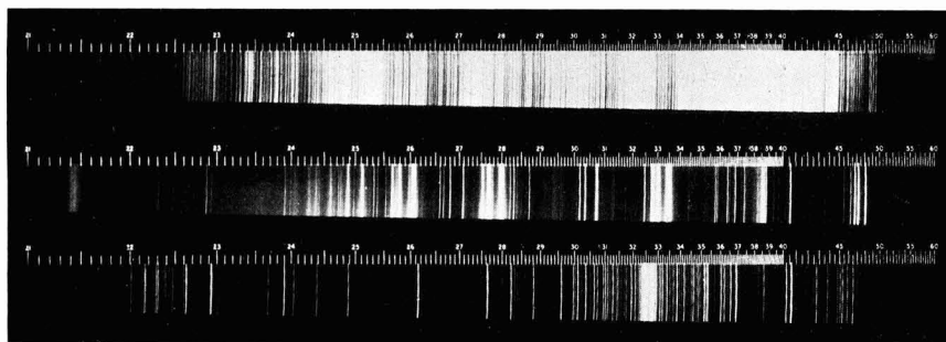
Fig. 2. Characteristic Spectra of Iron, Zinc and Copper Arcs.
