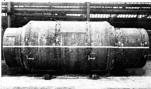
Mild Steel Rotary Kiln Shell 32' 5" long x 11' 10 \frac{1}{2} " diam. Manufactured by Messrs. Clayton for a cement works.
