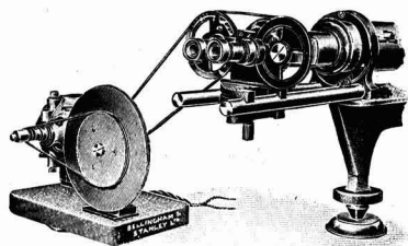
Fig. 5. Spectrograph equipped with Sector Photometer for Absorption Spectra.
