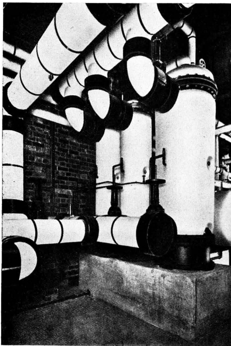
Insulation of Calorifiers and Pipework at the new Chemistry Buildings, Leeds University, with 85 per cent. Magnesia Sectional and Plastic Coverings supplied by the Chemical and Insulating Co., Ltd.
