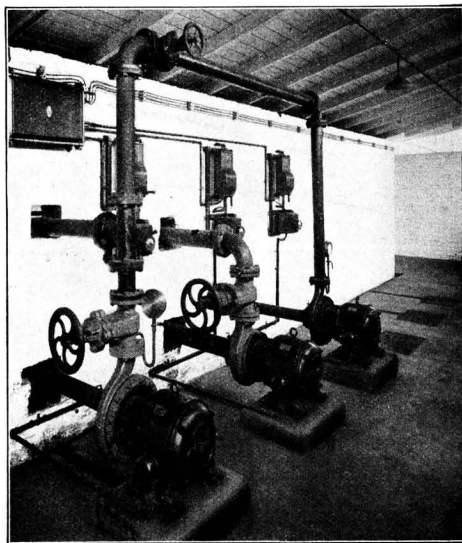
Three 3 in. Mopumps installed in a large Chemical Factory in the Midlands, with concrete foundations for three further pumps of the same size and type.
