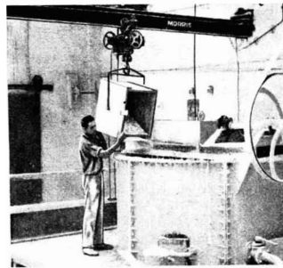
Left: This Morris Hoist is installed at a works where china clay is fed intermittently to a battery of mixers.
