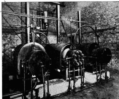
Front View of Bergius Converters.
