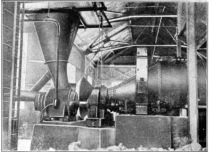
Hardinge Grinding Mill with Air Separation.
