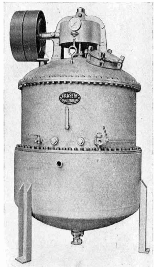
Fig. 5J (right).—Pressure Autoclave in "Staybrite" steel, 5 ft. diameter. (W. J. Fraser and Co., Ltd.)
