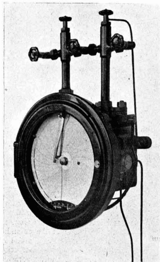
Modern Flow Controller, showing the pilot valve, on the side, to which the connecting pipes are directly attached. (Geo. Kent, Ltd.)
