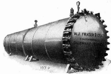
Fig. 3.—Large Horizontal Autoclave. (W. J. Fraser and Co., Ltd.)
