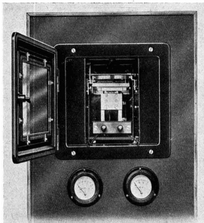
Pneumatic Controller for difference in temperature, with a potentiometer attachment giving a large range of temperature setting on the dial. Temperature is measured by thermocouples. (Geo. Kent, Ltd.)
