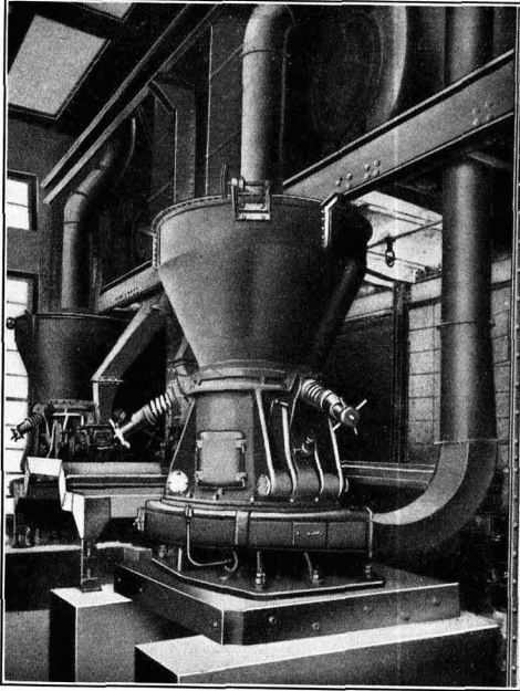
Raymond Lopulco Mill with Air Separation.
