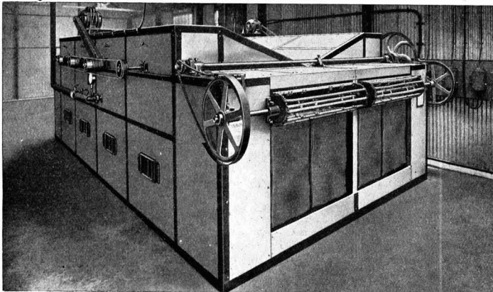
Fig. 2.—Tunnel stove capable of being arranged for steam, electric or gas heating.
