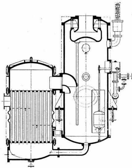
Vertical Section of "Hick Hargreaves" evaporator, with one calandria (on the left) and evaporator body (on the right) with safety valve, balanced piston valve controlled by a float and lever, steam separators and drier and hand-operated by-pass valve.
