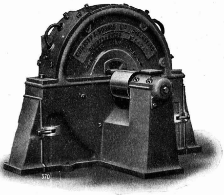
A Typical Disintegrating Plant. (Christy and Norris, Ltd.)
