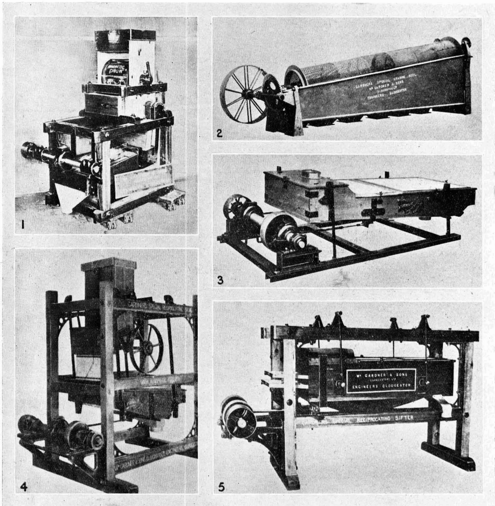
Fig. 1.—A Reciprocating Sieve Separator, with magnetic Drum fitted over for taking out foreign matter such as nails, filings, steel, etc.
