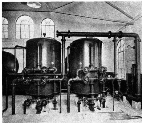
"Basex" Water Softening Plant at Shiplake with a capacity of 360,000 gallons per day.
