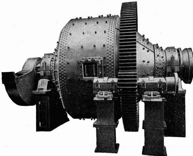
The photograph on the left shows a Hardinge Mill without Air Plant.
