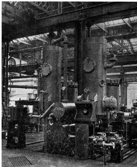
Typical Hick Hargreaves Evaporator assembled in the shops at Bolton.
