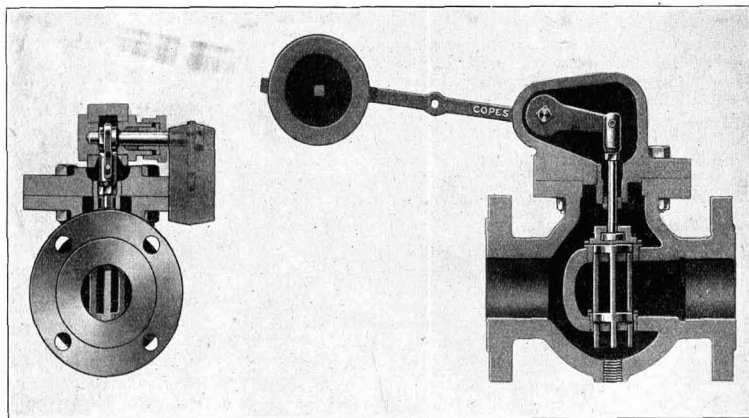
Copes's Control Valve showing low friction rotary spindle and high lift ported valve.
