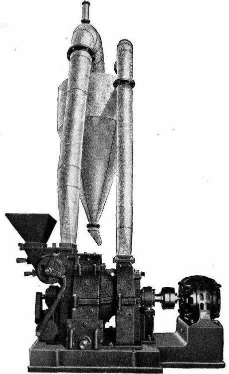
Raymond Impax Mill with Air Separation.
