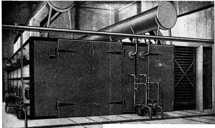
Fig. 3.—Hot Air Stove used for drying sacks, etc.
