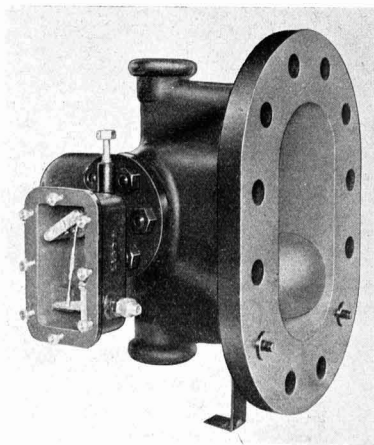
Pneumatic Level Regulator, showing the float, and the external pilot valve. (Geo. Kent, Ltd.)
