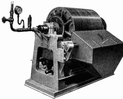
Fig. 1.—Film or Drum Dryer especially suitable for handling a liquid which cannot be filtered.
