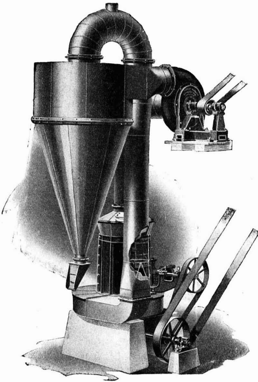
Raymond Mill equipped with Air Separation.
