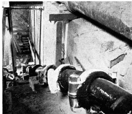
Steel Hydraulic Main, 6 in. diameter, fitted with "Victaulic" joints, in Leicester Square subway, London, illustrating the great flexibility of the pipe line.
