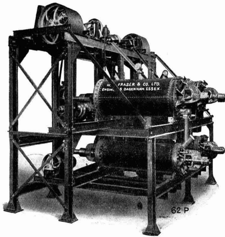
Fig. 1 (above).—Battery of Horizontal Autoclaves. (W. J. Fraser and Co., Ltd.)
