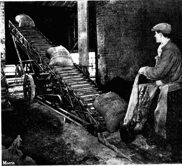
Above : This Morris Portable Conveyor is installed in a dockside warehouse. It is of the chain-lattice type.
