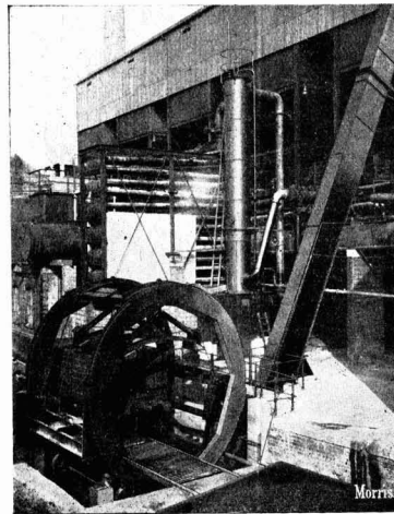
Above : A Morris Tippler working in conjunction with a Morris Elevator in handling coal.
