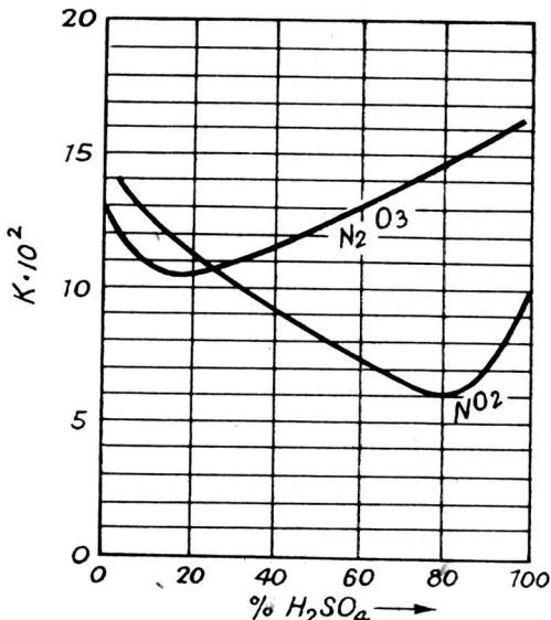
Fig. 2. Speed of absorption of N 2 O 3 and NO 2 in sulphuric acid
