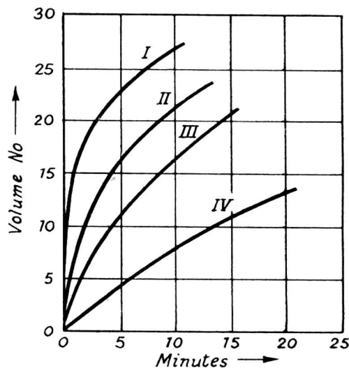
Fig. 4. Relative speed of reaction between SO_2 and nitrous sulphuric acid I-IV
