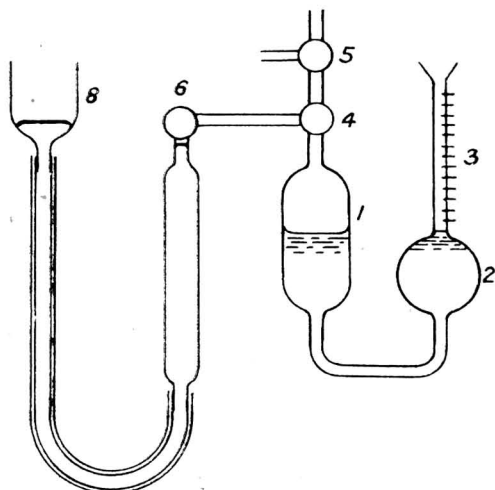
Fig. 3. Apparatus for the determination of relative reaction speed between SO_2 and nitrous sulphuric acid
