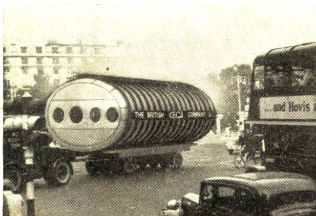
Stainless steel adsorber vessel passing Marble Arch. The vessel is one of three forming part of the largest automatic Solvent Recovery Plant in Europe now under construction in the United Kingdom.
