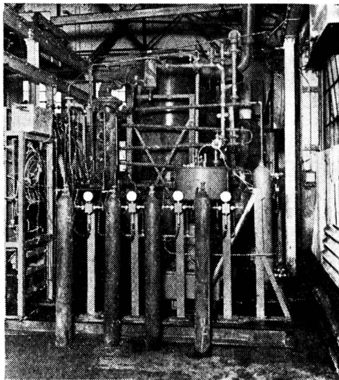
A Kestnamine CO 2 plant showing the charging header to which the gas cylinders are connected
