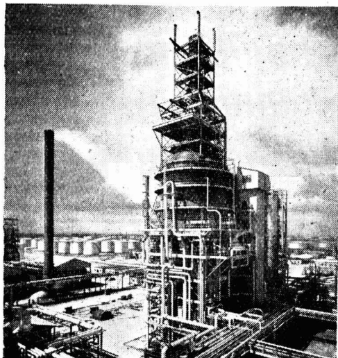
Completed catalytic cracking unit at Shell's Stanlow refinery
