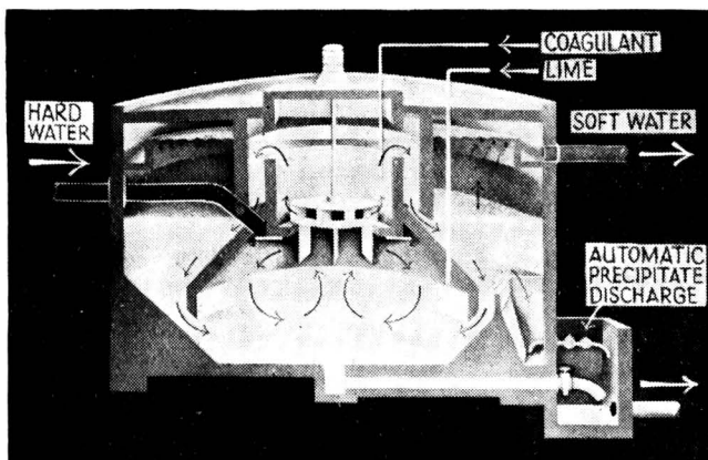
A diagram showing the interior of the 'Accelator' water softener
