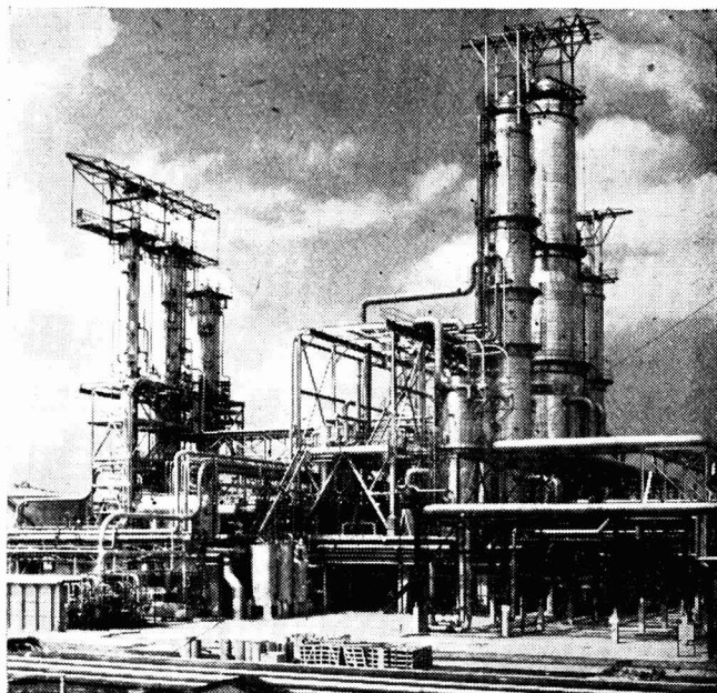
Distillation unit at Shell's Stanlow refinery
