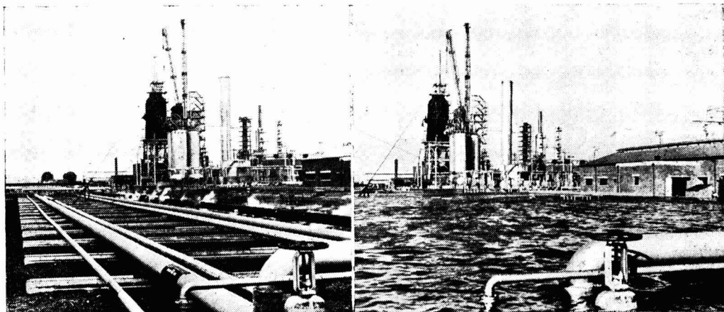
These photographs taken before and after recent flooding along the East coast of England show the main pipe track at the Anglo-Iranian's Isle of Grain refinery and illustrate the immense task now facing the management
