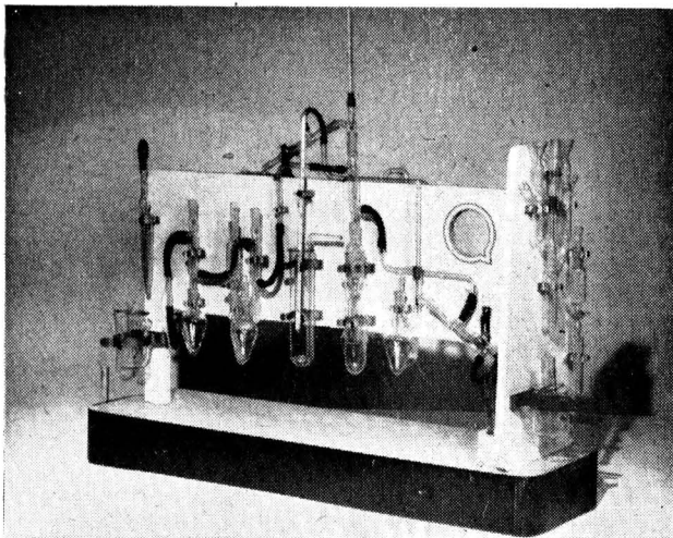
Side I of the assembly, and the end panel, showing the remarkable compactness of design.
