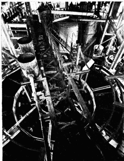
Phosphoric acid filter, with section of the phosphoric acid plant, at Marchon Products
