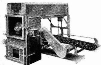
The "Adequate" Weigher shown with recorder doors open.
