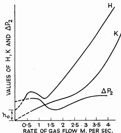
Fig. III Relation between working efficiency of plate and rate of gas flow
