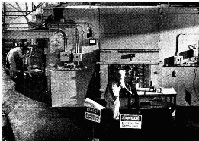
The 'Water Boiler' at the University of California's Los Alamos Scientific Laboratory was the first homogeneous reactor ever developed. It is used as a source of neutrons and for irradiation studies. Its fuel is uranyl nitrate enriched in uranium 235 and it operates at a power level of 35 kilowatts. Five more reactors are being designed or built at Los Alamos
