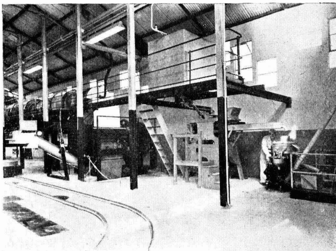
A view of one corner of the degreasing plant showing (bottom right) the receiver for the final product
