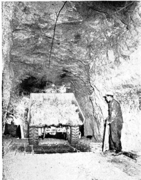
Anhydrite being dumped into a hopper in the mine for conveying to the surface
