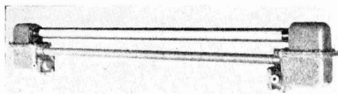
GEC flameproof fitting for 80 watt five ft. fluorescent lamp
