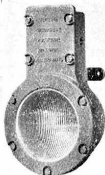
Holophane bulkhead flameproof unit No. F.9796 Buxton certified for use with inflammable gas in Groups 2 and 3. Designed for use with 60 - 100 - 150 watt GLS lamps
