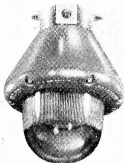
Holophane flameproof unit No. F.9821 for ceiling mounting. Lamp wattage 100-150 GLS Buxton certified under Class B (industrial type) for use in Groups 2 and 3 gases in the petroleum industry, cellulose plant, coal handling and treatment equipment areas and in a wide range of hazardous chemical processes. The body is of aluminium-silicon alloy casting, the front glass is a specially treated prismatic lens, and the reflector is an accurately moulded prismatic glass reflector arranged for close mounting to the lamp
