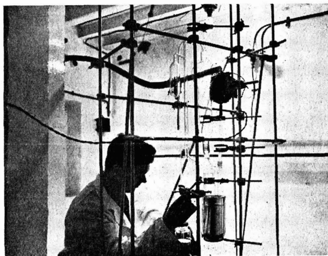
Equipment used in the study of a gas phase reaction under the influence of gamma radiation from the cobalt 60 source. The source tube can be seen passing through the annular reaction vessel
