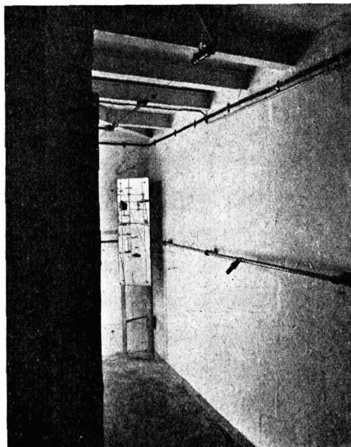
When the cobalt 60 source in the radiation laboratory is in the working area, visual observations can be made from outside the radiation shield by means of a series of mirrors and a telescope
