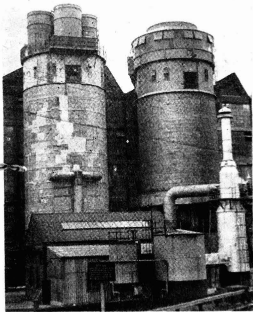
This picture shows the contrast between the two towers, both of which have had 18 months' exposure. The one on the left was coated with conventional paint, and the one on the right with the Epikote resin based system
