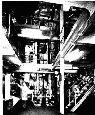
Fatty acid distillation plant of Price's (Bromborough)
