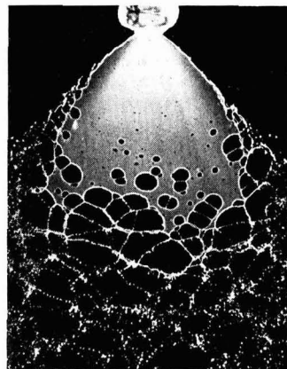
High speed photograph of a fan or flat spray nozzle, by H. T. Watson Ltd., shows mode of formation of drops. (1) Puncture of film causing holes with thick rims; (2) break up of rims into ligaments of liquid; (3) final break up of ligaments into drops
