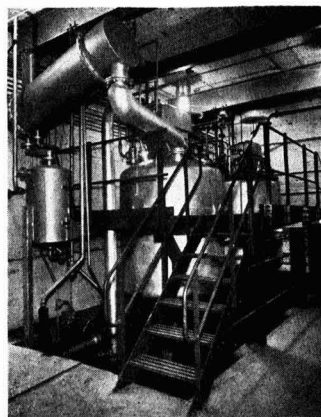
Pepton 22 plant reaction vessels of the Anchor Chemical Company
