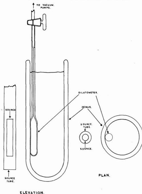
Fig. 1. Experimental arrangement for irradiation
