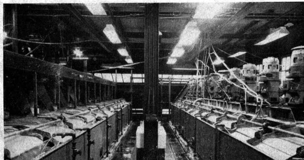
Flotation cells at Glebe Mines Limited, Eyam, Derbyshire, where fluorspar, barytes and lead are separated from the ore
