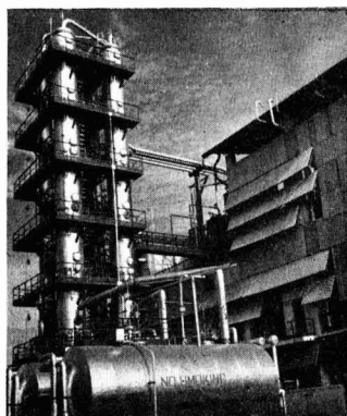
Benzol plant of the Bhilai steelworks
