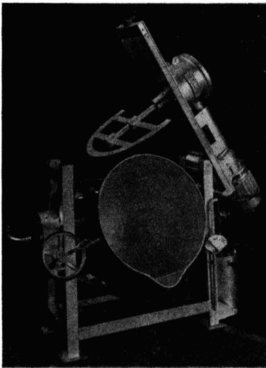
This Mixing Machine has Pan lined with Pure Silver. Type 23 PJ.
